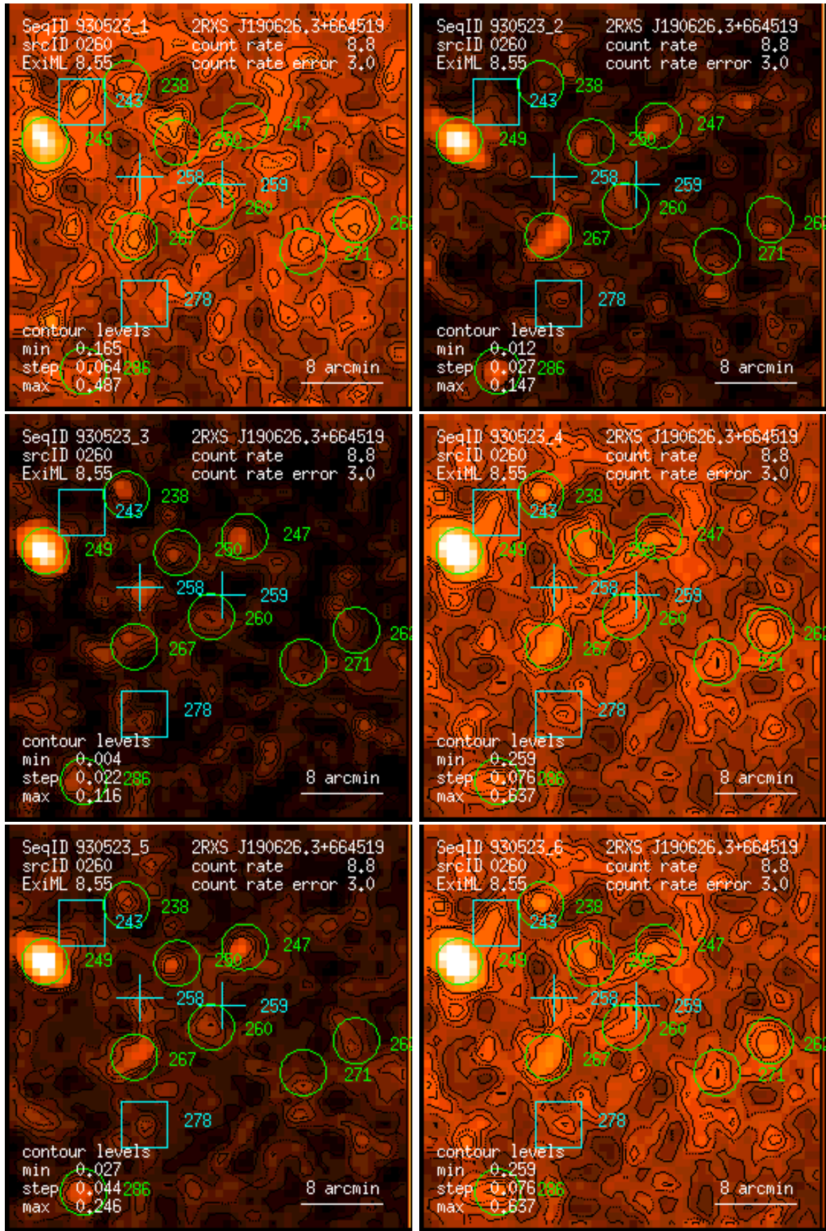
Figure 260: RASS 930523: detection 0260: band rate images, Gaussian filter: (1) PSPC channels 11 – 41, (2) 52 – 90, (3) 91 – 201, (4) 11 – 235, (5) 52 – 201, (6) 11 – 201. Broad band rates in counts/ks. Band rate contour levels in counts/ks/arcmin 2 .
