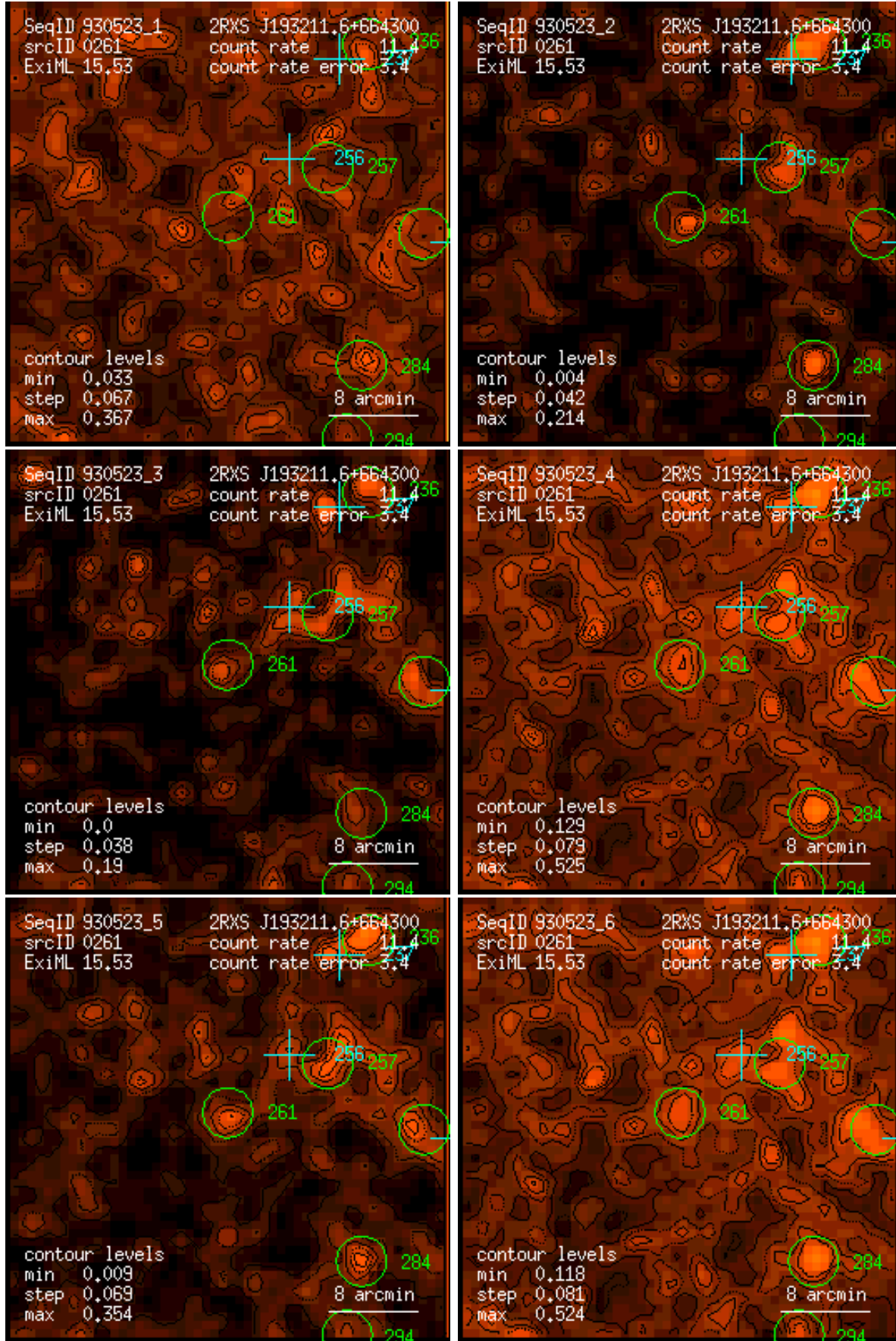
Figure 261: RASS 930523: detection 0261: band rate images, Gaussian filter: (1) PSPC channels 11 – 41, (2) 52 – 90, (3) 91 – 201, (4) 11 – 235, (5) 52 – 201, (6) 11 – 201. Broad band rates in counts/ks. Band rate contour levels in counts/ks/arcmin 2 .
