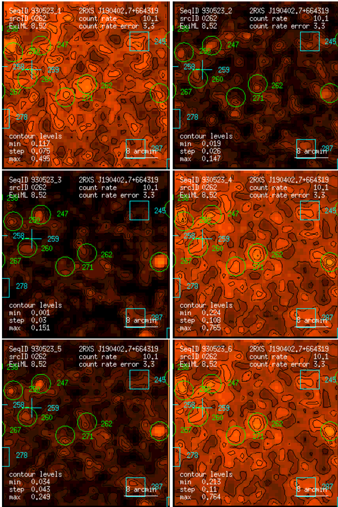
Figure 262: RASS 930523: detection 0262: band rate images, Gaussian filter: (1) PSPC channels 11 – 41, (2) 52 – 90, (3) 91 – 201, (4) 11 – 235, (5) 52 – 201, (6) 11 – 201. Broad band rates in counts/ks. Band rate contour levels in counts/ks/arcmin 2 .
