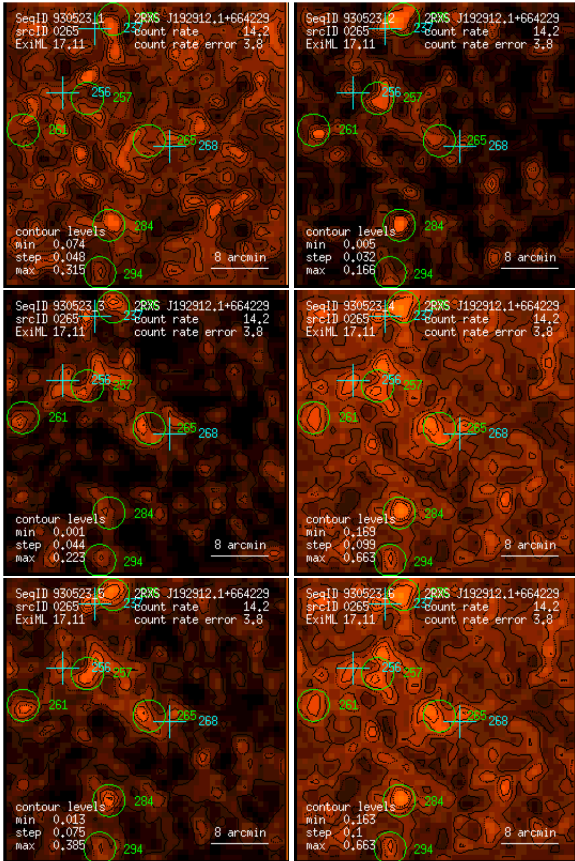
Figure 265: RASS 930523: detection 0265: band rate images, Gaussian filter: (1) PSPC channels 11 – 41, (2) 52 – 90, (3) 91 – 201, (4) 11 – 235, (5) 52 – 201, (6) 11 – 201. Broad band rates in counts/ks. Band rate contour levels in counts/ks/arcmin 2 .
