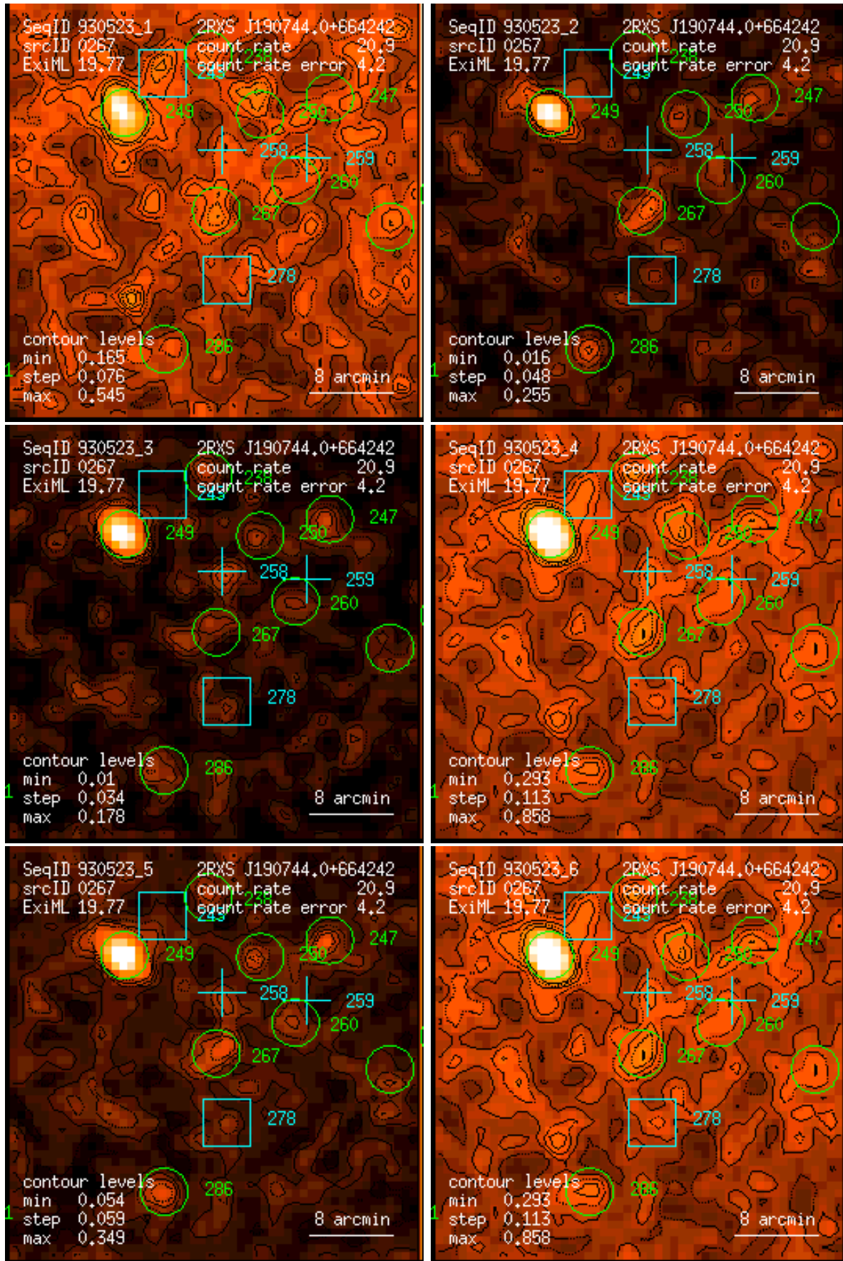
Figure 267: RASS 930523: detection 0267: band rate images, Gaussian filter: (1) PSPC channels 11 – 41, (2) 52 – 90, (3) 91 – 201, (4) 11 – 235, (5) 52 – 201, (6) 11 – 201. Broad band rates in counts/ks. Band rate contour levels in counts/ks/arcmin 2 .
