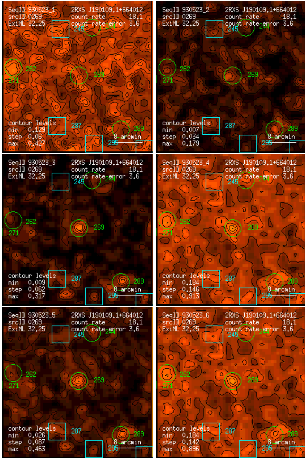
Figure 269: RASS 930523: detection 0269: band rate images, Gaussian filter: (1) PSPC channels 11 – 41, (2) 52 – 90, (3) 91 – 201, (4) 11 – 235, (5) 52 – 201, (6) 11 – 201. Broad band rates in counts/ks. Band rate contour levels in counts/ks/arcmin 2 .
