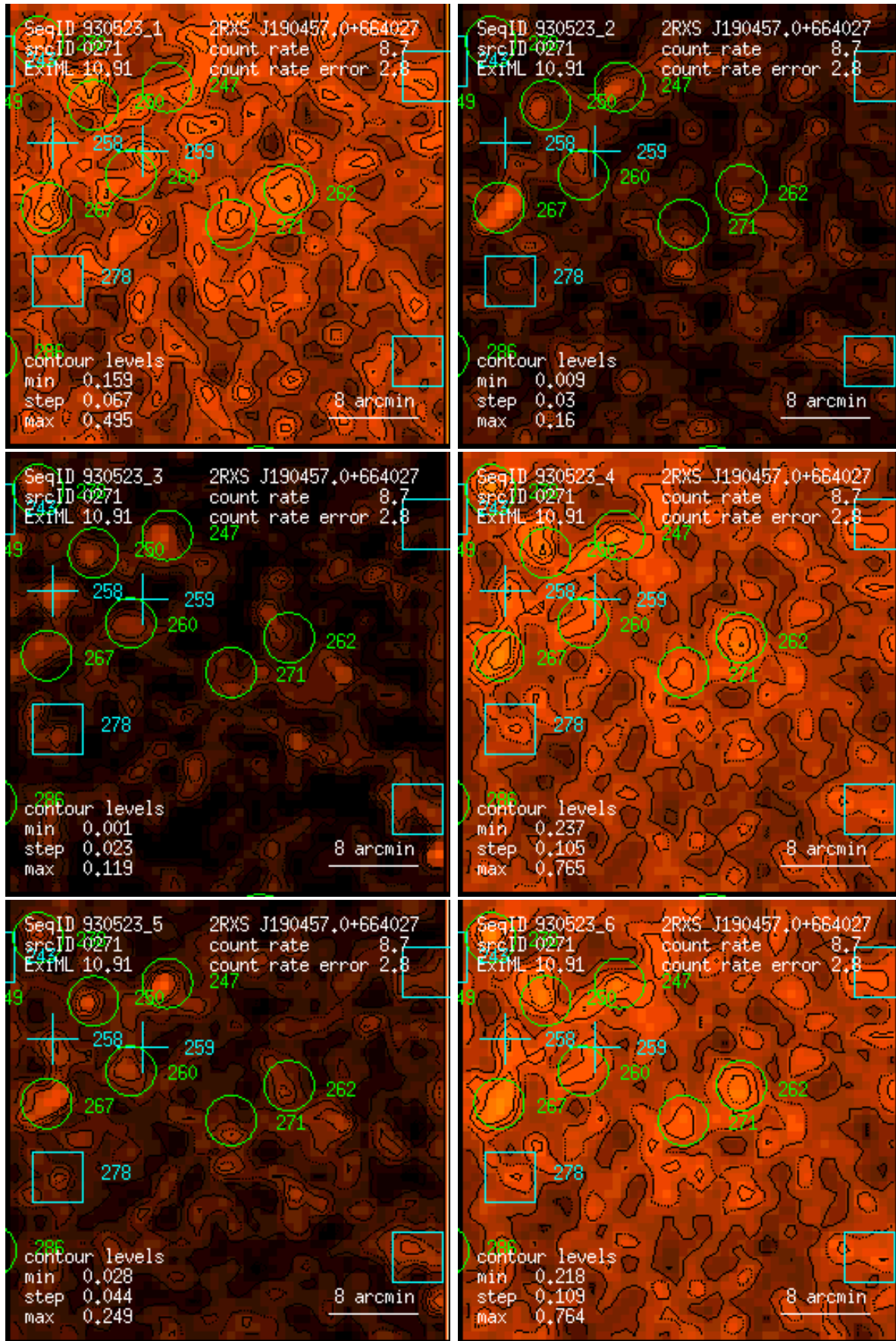
Figure 271: RASS 930523: detection 0271: band rate images, Gaussian filter: (1) PSPC channels 11 – 41, (2) 52 – 90, (3) 91 – 201, (4) 11 – 235, (5) 52 – 201, (6) 11 – 201. Broad band rates in counts/ks. Band rate contour levels in counts/ks/arcmin 2 .
