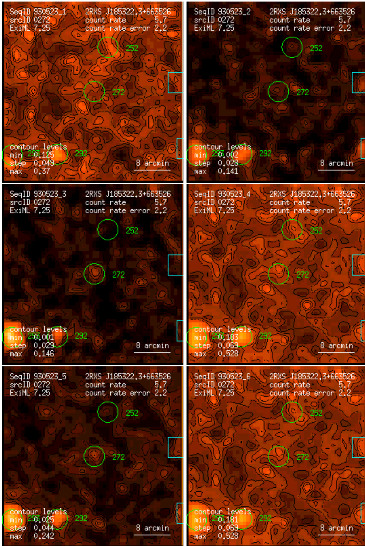
Figure 272: RASS 930523: detection 0272: band rate images, Gaussian filter: (1) PSPC channels 11 – 41, (2) 52 – 90, (3) 91 – 201, (4) 11 – 235, (5) 52 – 201, (6) 11 – 201. Broad band rates in counts/ks. Band rate contour levels in counts/ks/arcmin 2 .
