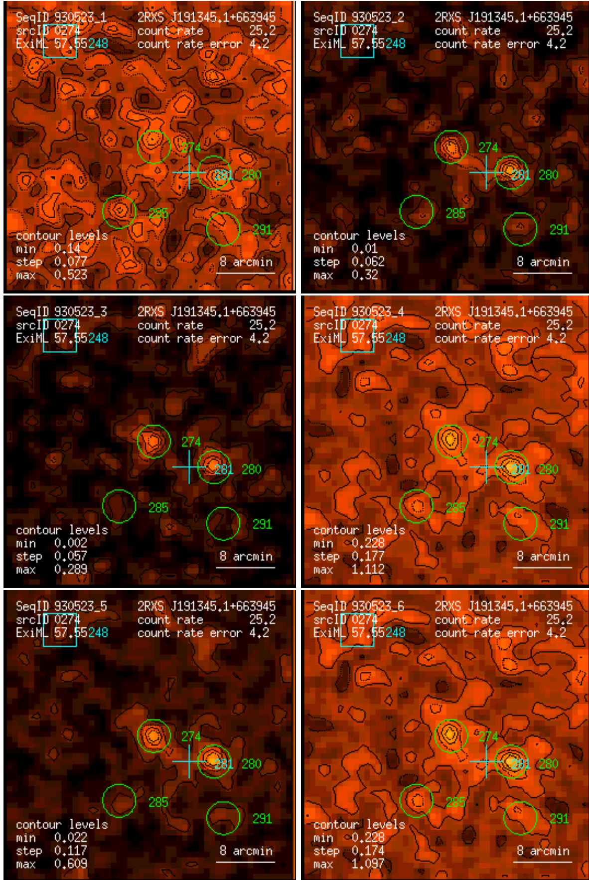
Figure 274: RASS 930523: detection 0274: band rate images, Gaussian filter: (1) PSPC channels 11 – 41, (2) 52 – 90, (3) 91 – 201, (4) 11 – 235, (5) 52 – 201, (6) 11 – 201. Broad band rates in counts/ks. Band rate contour levels in counts/ks/arcmin 2 .
