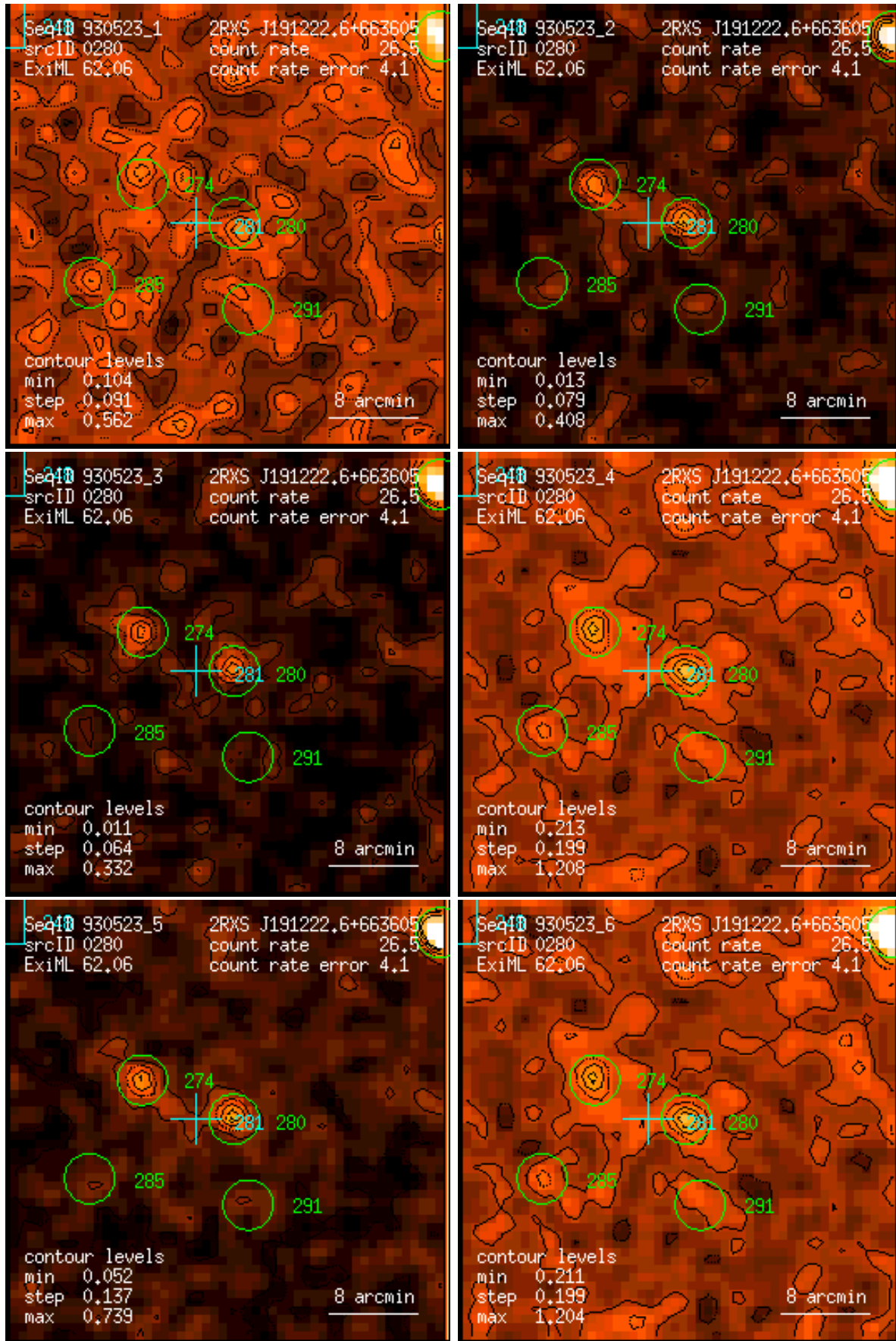
Figure 280: RASS 930523: detection 0280: band rate images, Gaussian filter: (1) PSPC channels 11 – 41, (2) 52 – 90, (3) 91 – 201, (4) 11 – 235, (5) 52 – 201, (6) 11 – 201. Broad band rates in counts/ks. Band rate contour levels in counts/ks/arcmin 2 .
