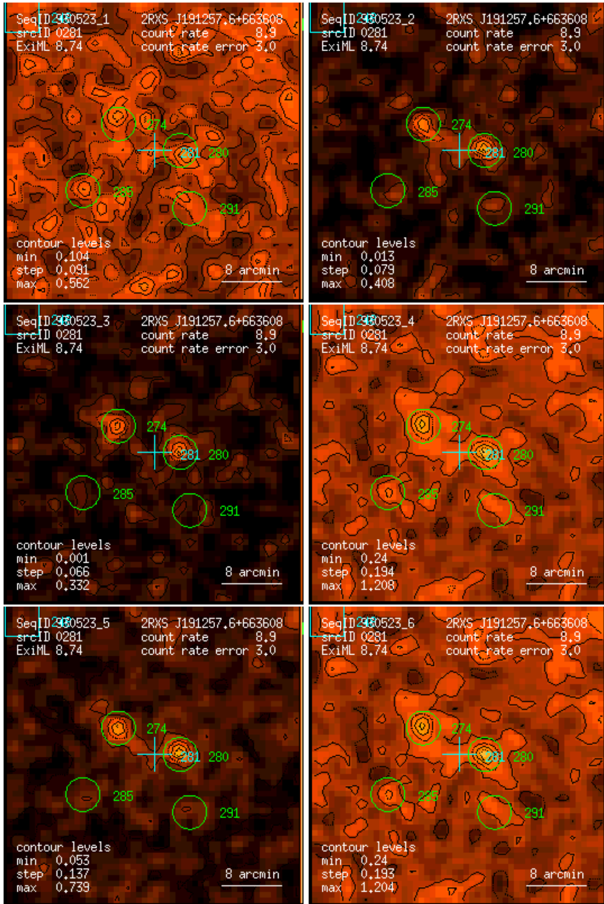
Figure 281: RASS 930523: detection 0281: band rate images, Gaussian filter: (1) PSPC channels 11 – 41, (2) 52 – 90, (3) 91 – 201, (4) 11 – 235, (5) 52 – 201, (6) 11 – 201. Broad band rates in counts/ks. Band rate contour levels in counts/ks/arcmin 2 .
