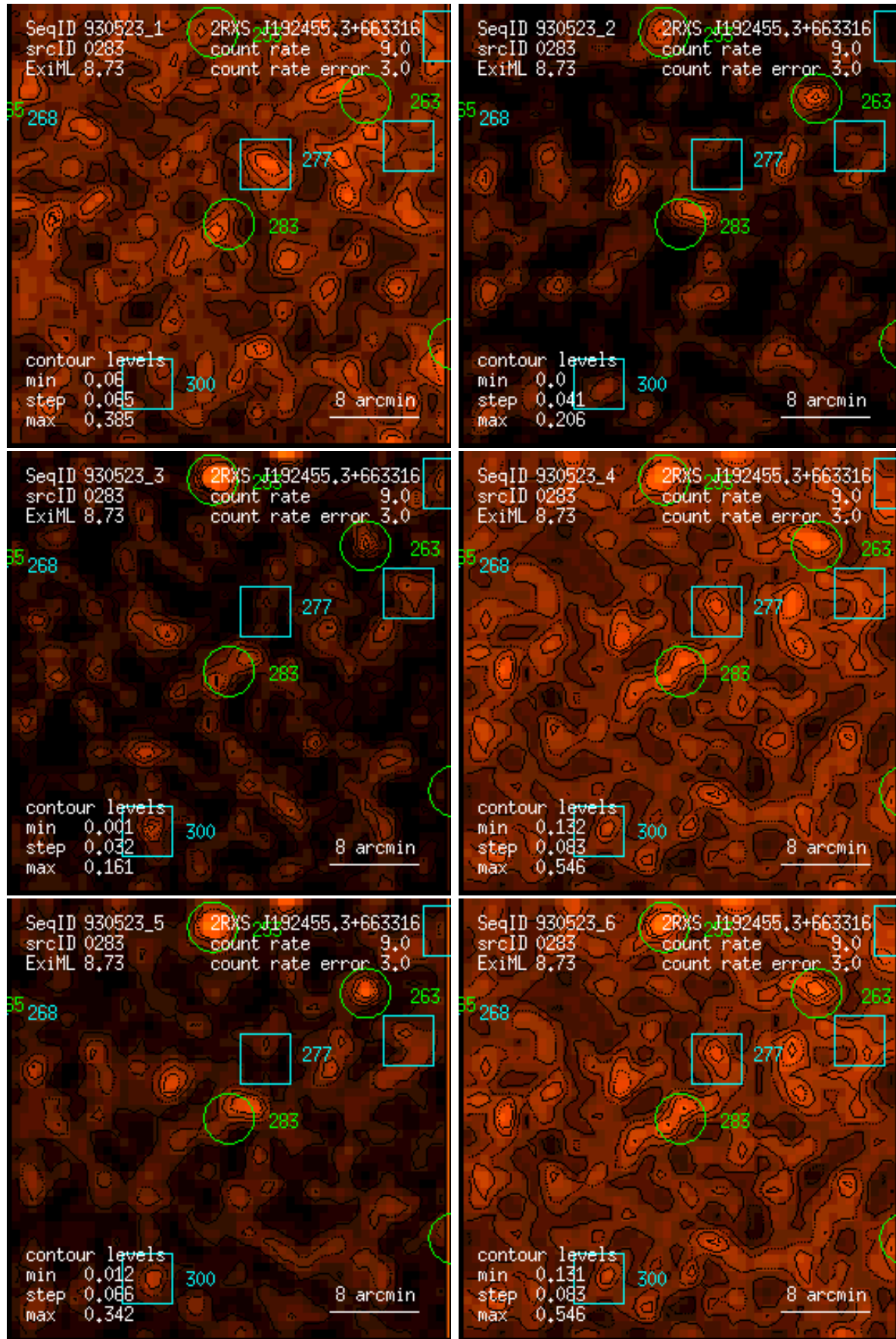
Figure 283: RASS 930523: detection 0283: band rate images, Gaussian filter: (1) PSPC channels 11 – 41, (2) 52 – 90, (3) 91 – 201, (4) 11 – 235, (5) 52 – 201, (6) 11 – 201. Broad band rates in counts/ks. Band rate contour levels in counts/ks/arcmin 2 .
