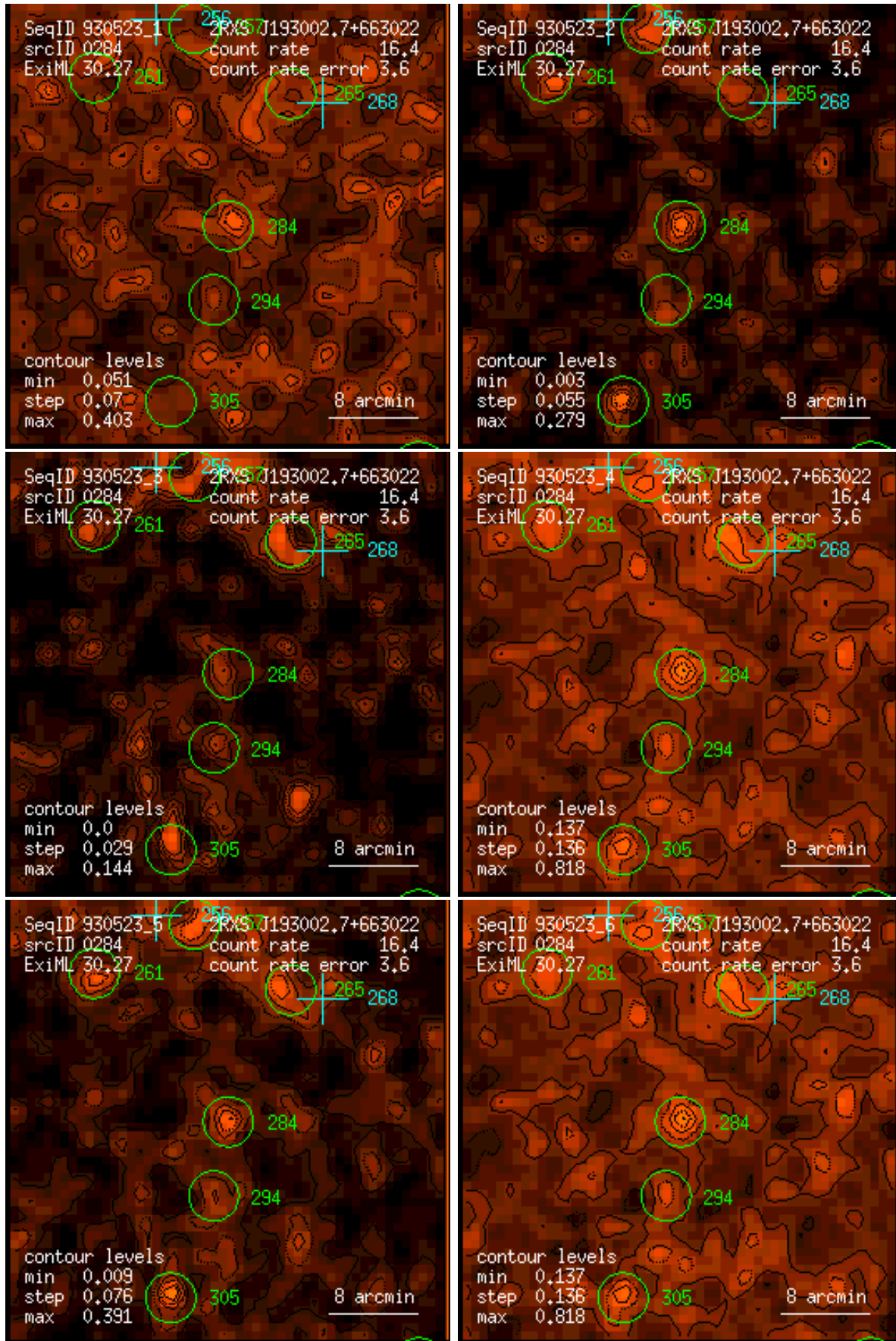
Figure 284: RASS 930523: detection 0284: band rate images, Gaussian filter: (1) PSPC channels 11 – 41, (2) 52 – 90, (3) 91 – 201, (4) 11 – 235, (5) 52 – 201, (6) 11 – 201. Broad band rates in counts/ks. Band rate contour levels in counts/ks/arcmin 2 .
