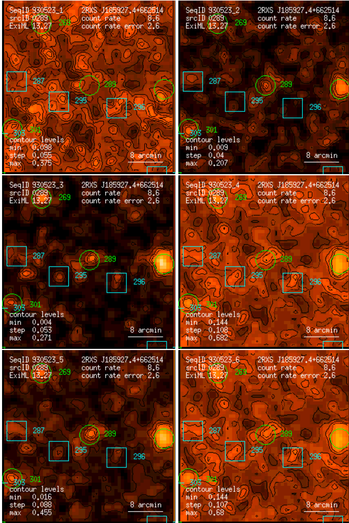
Figure 289: RASS 930523: detection 0289: band rate images, Gaussian filter: (1) PSPC channels 11 – 41, (2) 52 – 90, (3) 91 – 201, (4) 11 – 235, (5) 52 – 201, (6) 11 – 201. Broad band rates in counts/ks. Band rate contour levels in counts/ks/arcmin 2 .
