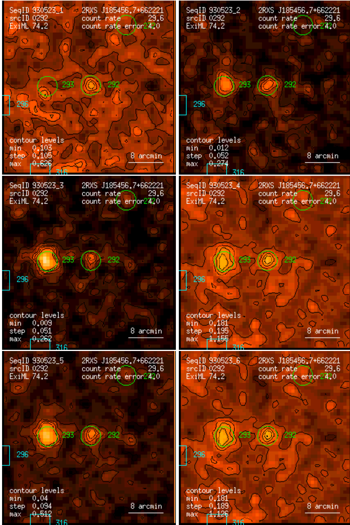
Figure 292: RASS 930523: detection 0292: band rate images, Gaussian filter: (1) PSPC channels 11 – 41, (2) 52 – 90, (3) 91 – 201, (4) 11 – 235, (5) 52 – 201, (6) 11 – 201. Broad band rates in counts/ks. Band rate contour levels in counts/ks/arcmin 2 .
