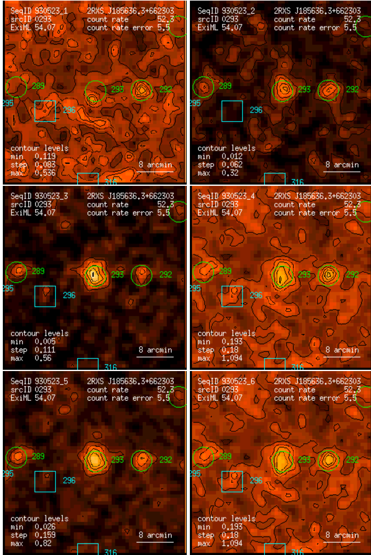
Figure 293: RASS 930523: detection 0293: band rate images, Gaussian filter: (1) PSPC channels 11 – 41, (2) 52 – 90, (3) 91 – 201, (4) 11 – 235, (5) 52 – 201, (6) 11 – 201. Broad band rates in counts/ks. Band rate contour levels in counts/ks/arcmin 2 .
