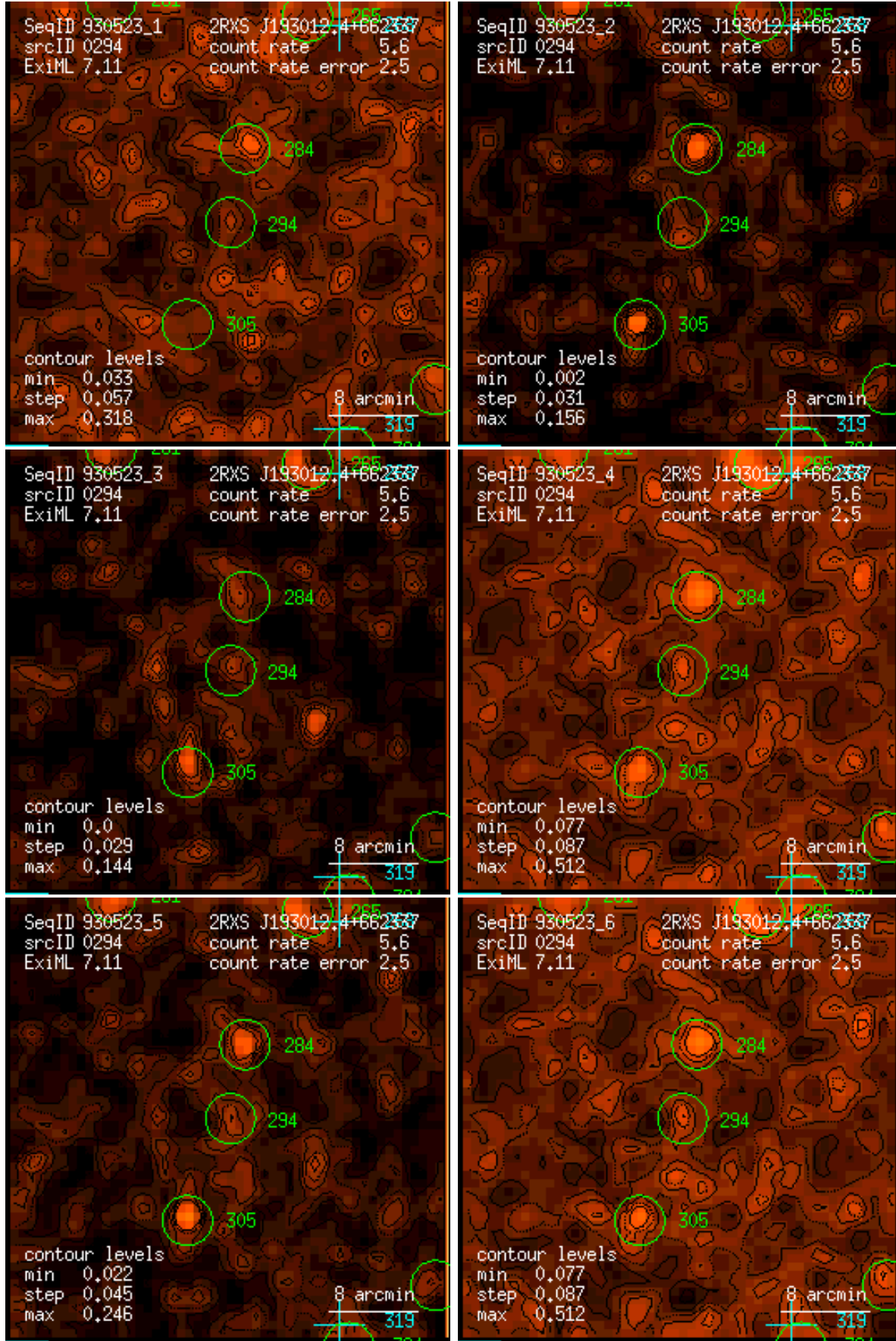
Figure 294: RASS 930523: detection 0294: band rate images, Gaussian filter: (1) PSPC channels 11 – 41, (2) 52 – 90, (3) 91 – 201, (4) 11 – 235, (5) 52 – 201, (6) 11 – 201. Broad band rates in counts/ks. Band rate contour levels in counts/ks/arcmin 2 .
