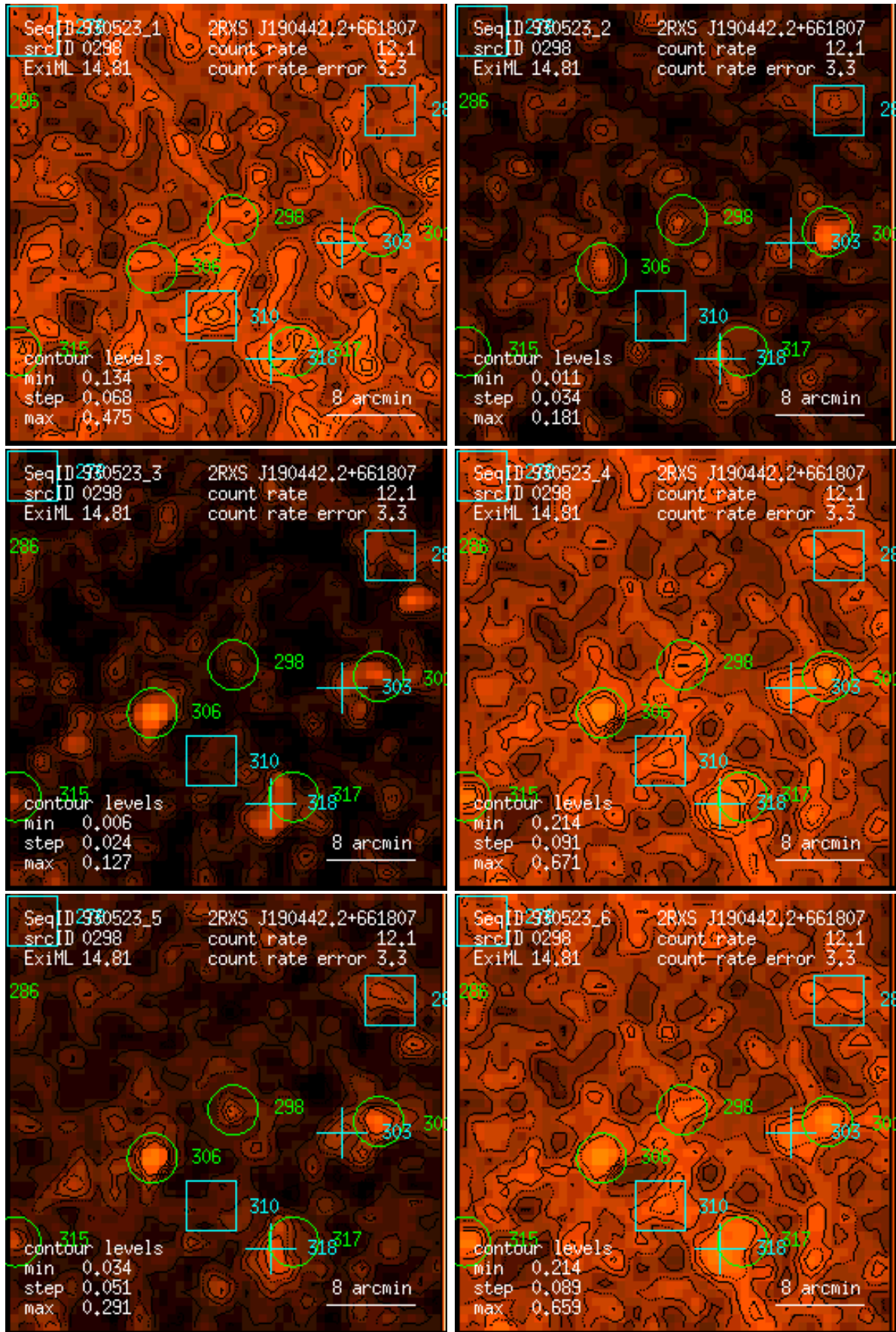
Figure 298: RASS 930523: detection 0298: band rate images, Gaussian filter: (1) PSPC channels 11 – 41, (2) 52 – 90, (3) 91 – 201, (4) 11 – 235, (5) 52 – 201, (6) 11 – 201. Broad band rates in counts/ks. Band rate contour levels in counts/ks/arcmin 2 .
