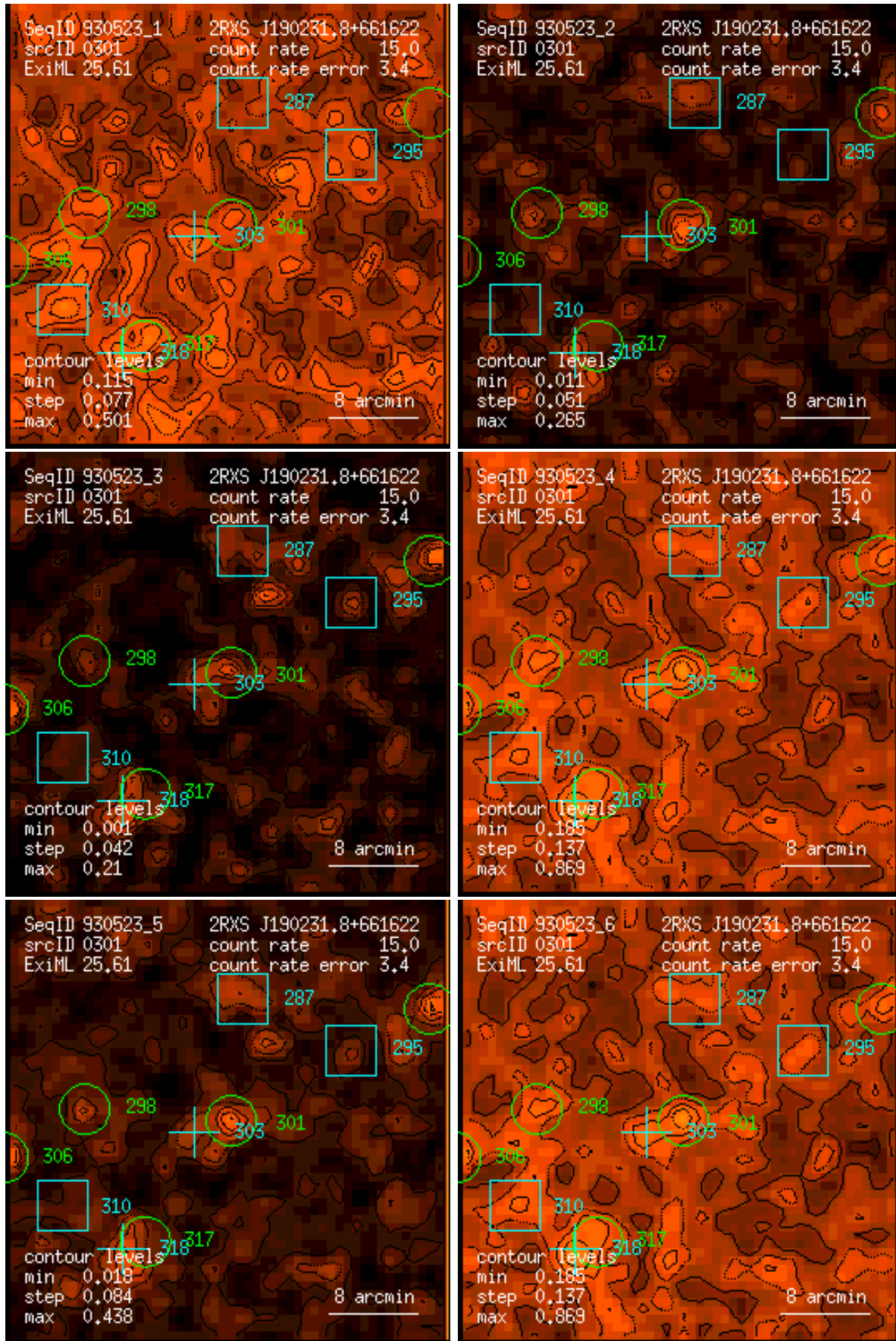
Figure 301: RASS 930523: detection 0301: band rate images, Gaussian filter: (1) PSPC channels 11 – 41, (2) 52 – 90, (3) 91 – 201, (4) 11 – 235, (5) 52 – 201, (6) 11 – 201. Broad band rates in counts/ks. Band rate contour levels in counts/ks/arcmin 2 .
