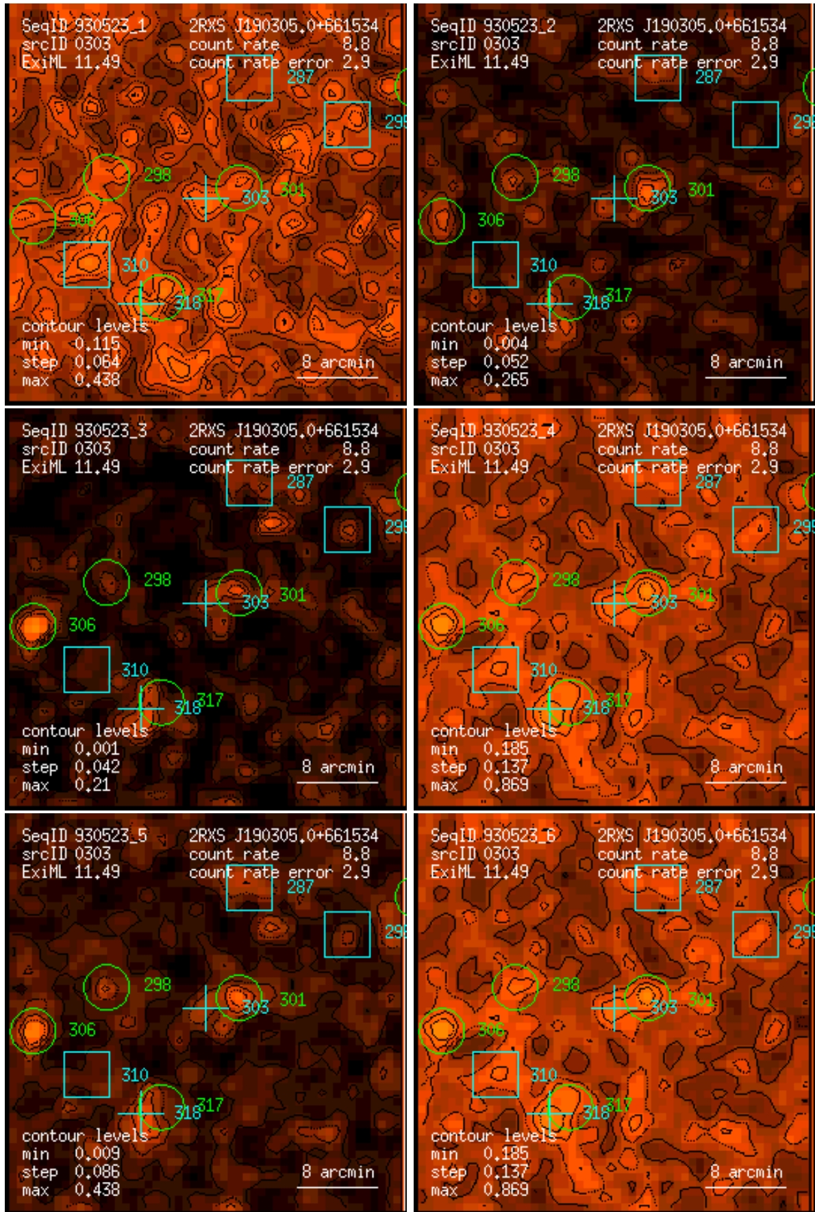
Figure 303: RASS 930523: detection 0303: band rate images, Gaussian filter: (1) PSPC channels 11 – 41, (2) 52 – 90, (3) 91 – 201, (4) 11 – 235, (5) 52 – 201, (6) 11 – 201. Broad band rates in counts/ks. Band rate contour levels in counts/ks/arcmin 2 .
