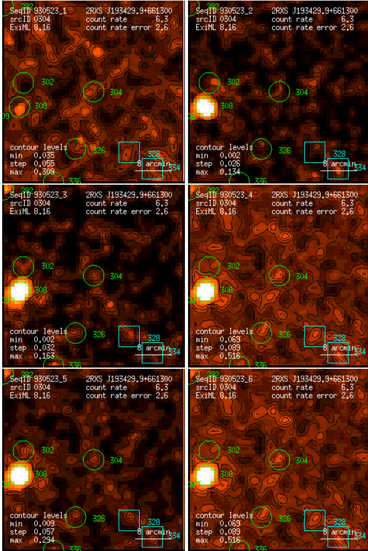
Figure 304: RASS 930523: detection 0304: band rate images, Gaussian filter: (1) PSPC channels 11 – 41, (2) 52 – 90, (3) 91 – 201, (4) 11 – 235, (5) 52 – 201, (6) 11 – 201. Broad band rates in counts/ks. Band rate contour levels in counts/ks/arcmin 2 .
