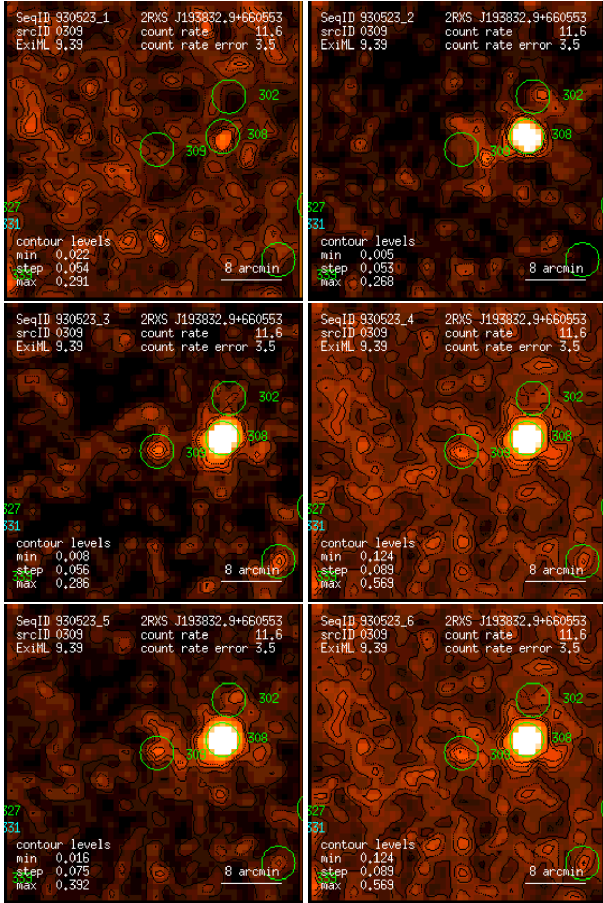
Figure 309: RASS 930523: detection 0309: band rate images, Gaussian filter: (1) PSPC channels 11 – 41, (2) 52 – 90, (3) 91 – 201, (4) 11 – 235, (5) 52 – 201, (6) 11 – 201. Broad band rates in counts/ks. Band rate contour levels in counts/ks/arcmin 2 .
