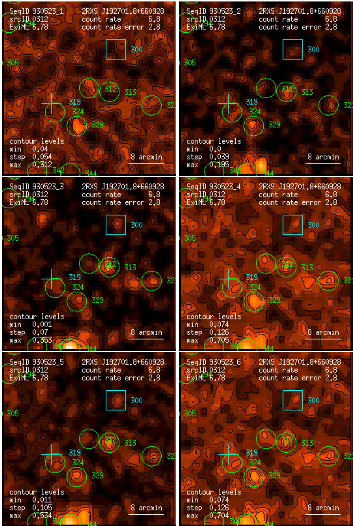
Figure 312: RASS 930523: detection 0312: band rate images, Gaussian filter: (1) PSPC channels 11 – 41, (2) 52 – 90, (3) 91 – 201, (4) 11 – 235, (5) 52 – 201, (6) 11 – 201. Broad band rates in counts/ks. Band rate contour levels in counts/ks/arcmin 2 .
