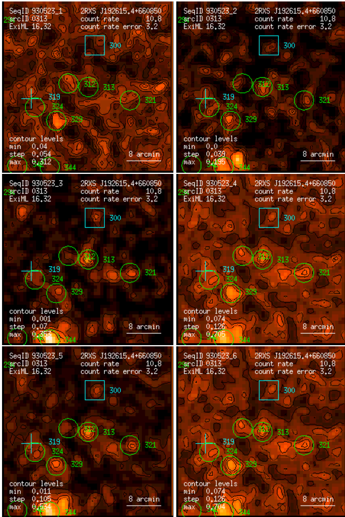
Figure 313: RASS 930523: detection 0313: band rate images, Gaussian filter: (1) PSPC channels 11 – 41, (2) 52 – 90, (3) 91 – 201, (4) 11 – 235, (5) 52 – 201, (6) 11 – 201. Broad band rates in counts/ks. Band rate contour levels in counts/ks/arcmin 2 .
