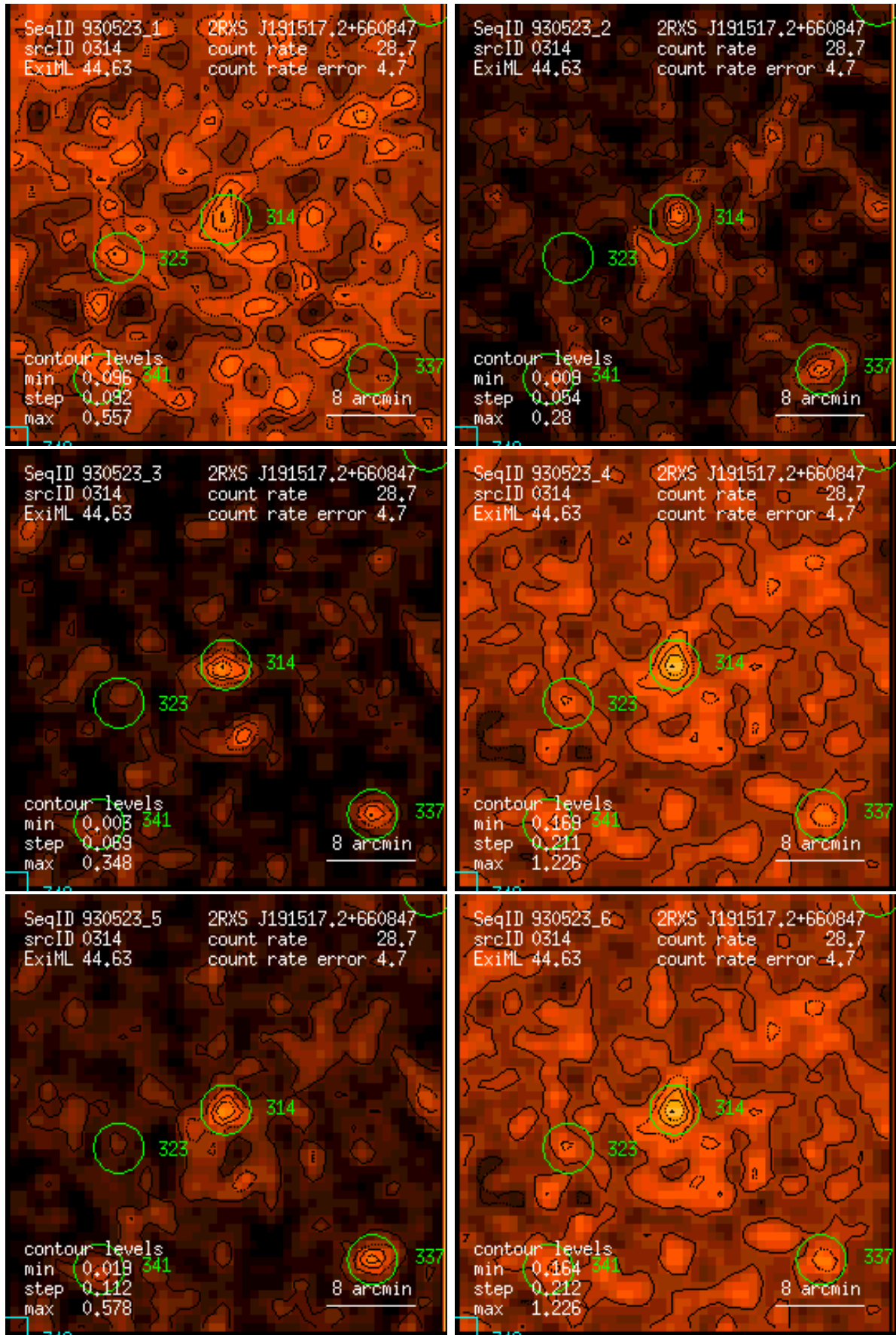
Figure 314: RASS 930523: detection 0314: band rate images, Gaussian filter: (1) PSPC channels 11 – 41, (2) 52 – 90, (3) 91 – 201, (4) 11 – 235, (5) 52 – 201, (6) 11 – 201. Broad band rates in counts/ks. Band rate contour levels in counts/ks/arcmin 2 .
