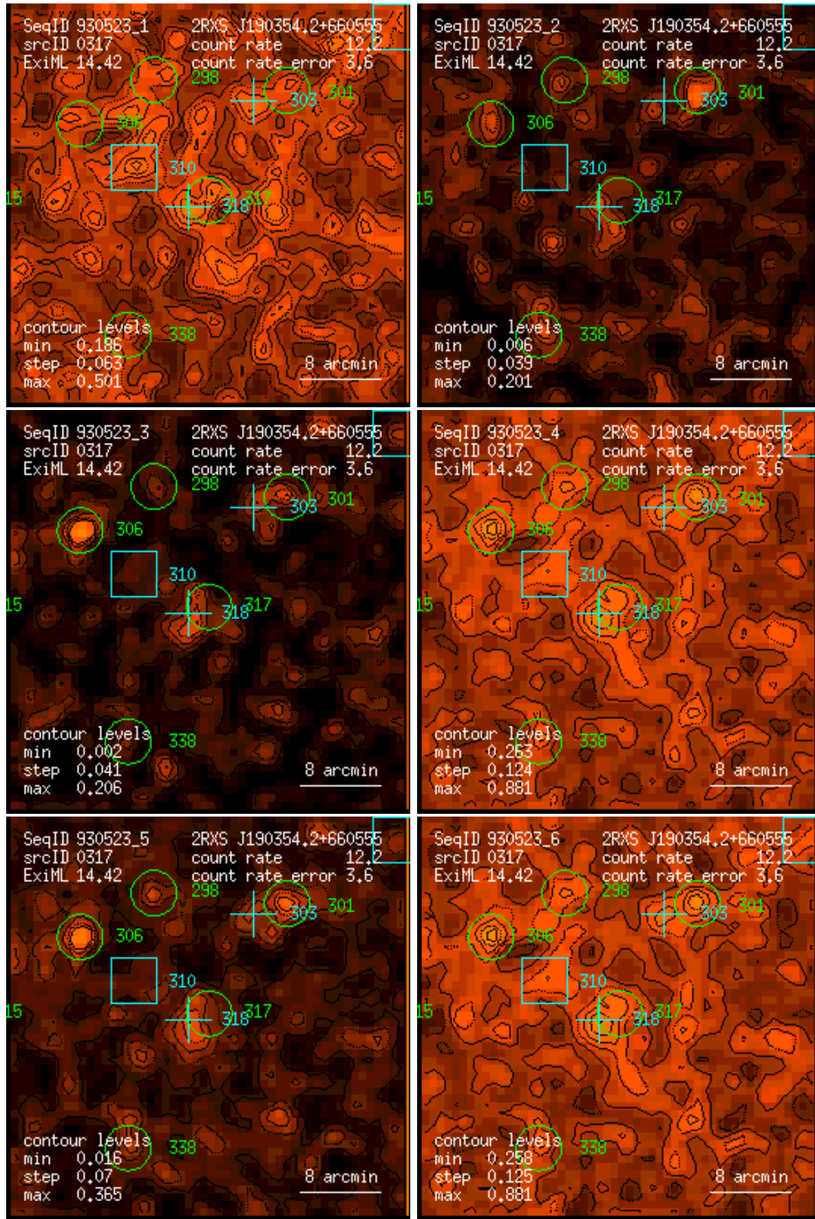
Figure 317: RASS 930523: detection 0317: band rate images, Gaussian filter: (1) PSPC channels 11 – 41, (2) 52 – 90, (3) 91 – 201, (4) 11 – 235, (5) 52 – 201, (6) 11 – 201. Broad band rates in counts/ks. Band rate contour levels in counts/ks/arcmin 2 .
