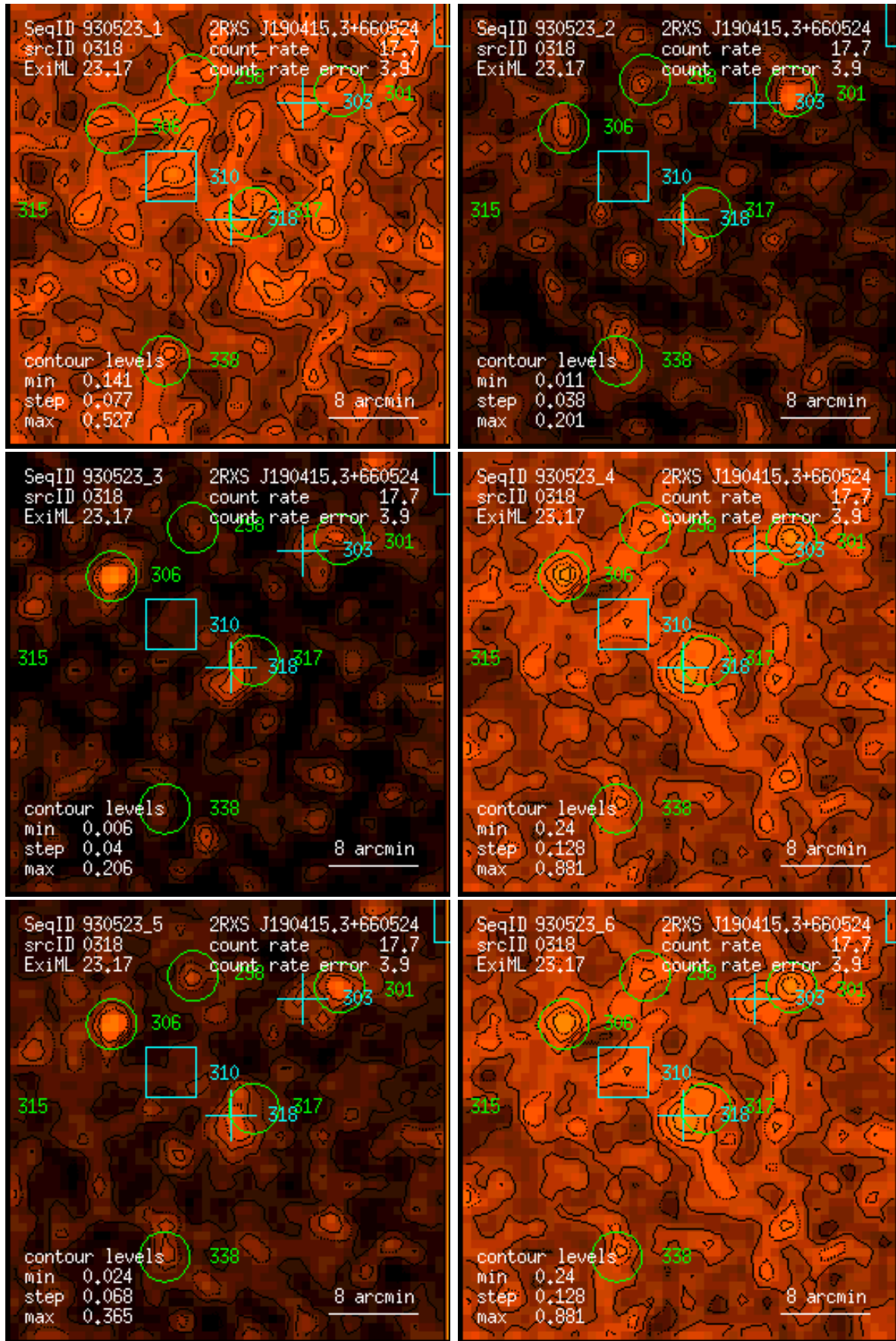
Figure 318: RASS 930523: detection 0318: band rate images, Gaussian filter: (1) PSPC channels 11 – 41, (2) 52 – 90, (3) 91 – 201, (4) 11 – 235, (5) 52 – 201, (6) 11 – 201. Broad band rates in counts/ks. Band rate contour levels in counts/ks/arcmin 2 .
