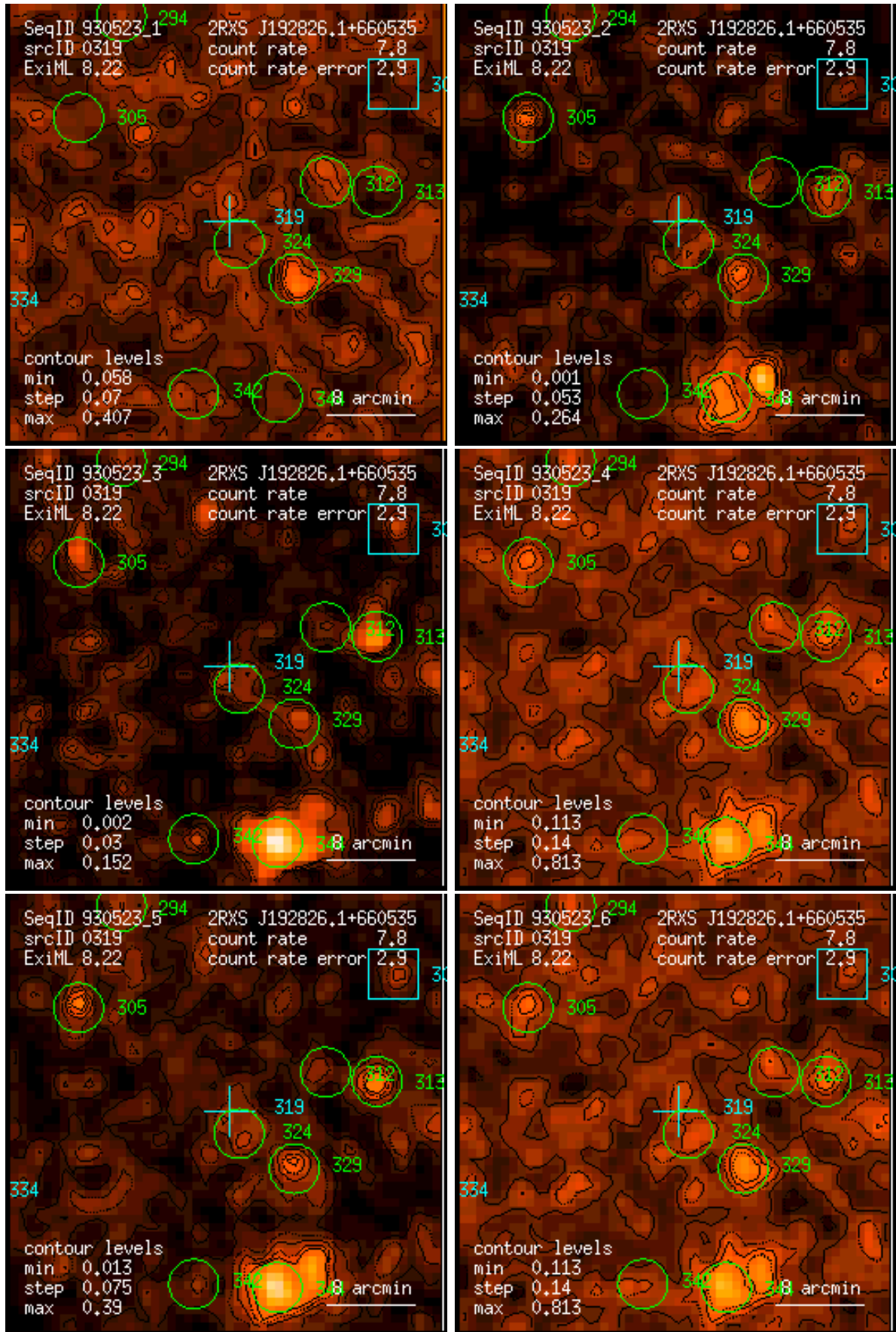
Figure 319: RASS 930523: detection 0319: band rate images, Gaussian filter: (1) PSPC channels 11 – 41, (2) 52 – 90, (3) 91 – 201, (4) 11 – 235, (5) 52 – 201, (6) 11 – 201. Broad band rates in counts/ks. Band rate contour levels in counts/ks/arcmin 2 .
