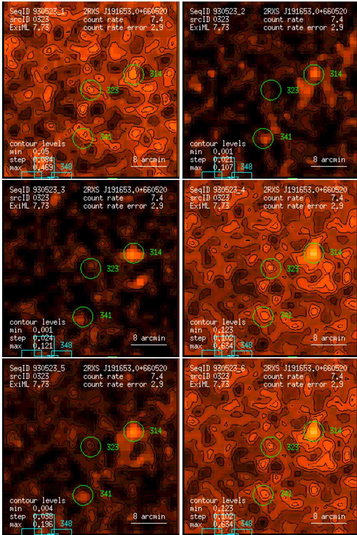
Figure 323: RASS 930523: detection 0323: band rate images, Gaussian filter: (1) PSPC channels 11 – 41, (2) 52 – 90, (3) 91 – 201, (4) 11 – 235, (5) 52 – 201, (6) 11 – 201. Broad band rates in counts/ks. Band rate contour levels in counts/ks/arcmin 2 .
