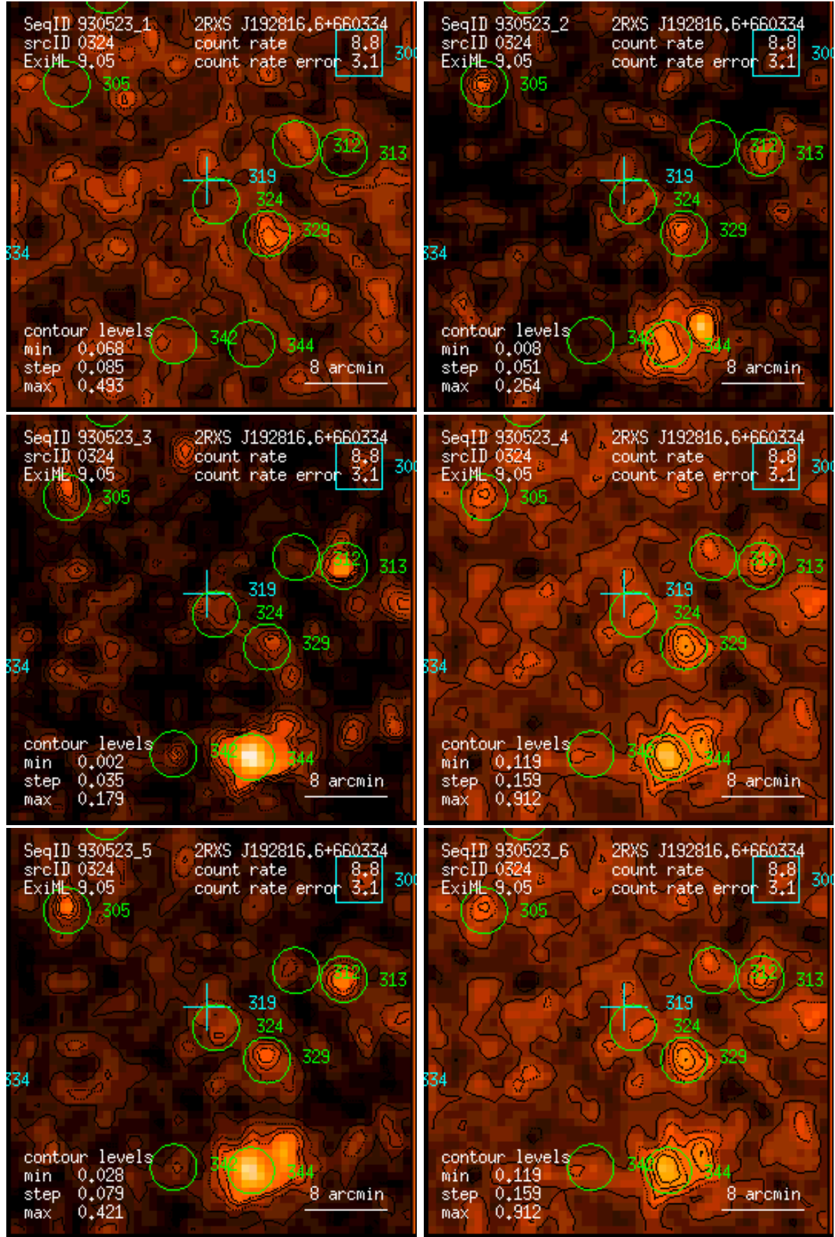
Figure 324: RASS 930523: detection 0324: band rate images, Gaussian filter: (1) PSPC channels 11 – 41, (2) 52 – 90, (3) 91 – 201, (4) 11 – 235, (5) 52 – 201, (6) 11 – 201. Broad band rates in counts/ks. Band rate contour levels in counts/ks/arcmin 2 .
