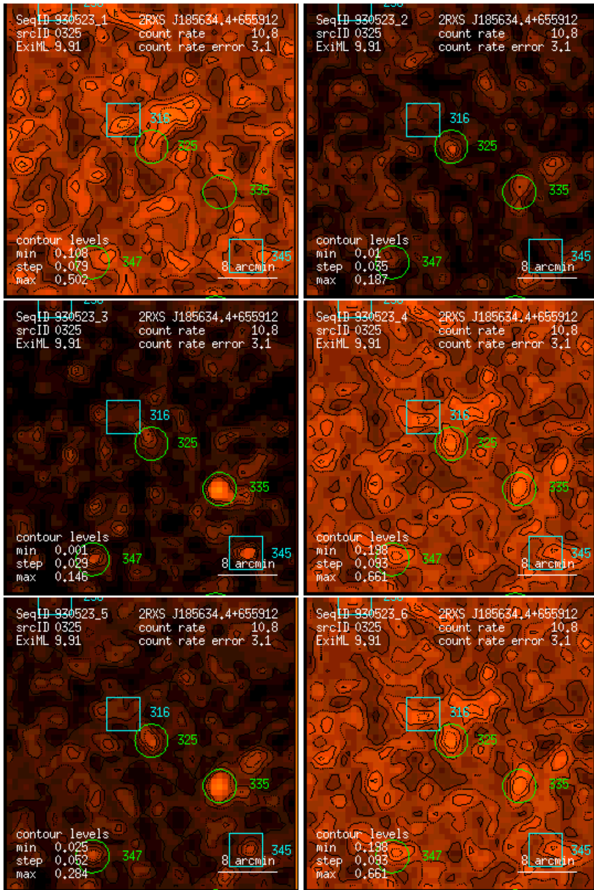
Figure 325: RASS 930523: detection 0325: band rate images, Gaussian filter: (1) PSPC channels 11 – 41, (2) 52 – 90, (3) 91 – 201, (4) 11 – 235, (5) 52 – 201, (6) 11 – 201. Broad band rates in counts/ks. Band rate contour levels in counts/ks/arcmin 2 .
