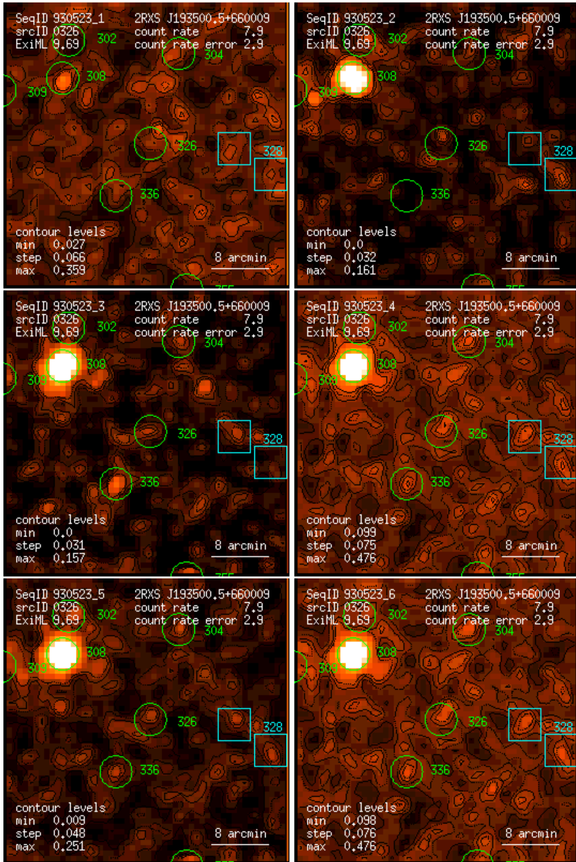
Figure 326: RASS 930523: detection 0326: band rate images, Gaussian filter: (1) PSPC channels 11 – 41, (2) 52 – 90, (3) 91 – 201, (4) 11 – 235, (5) 52 – 201, (6) 11 – 201. Broad band rates in counts/ks. Band rate contour levels in counts/ks/arcmin 2 .
