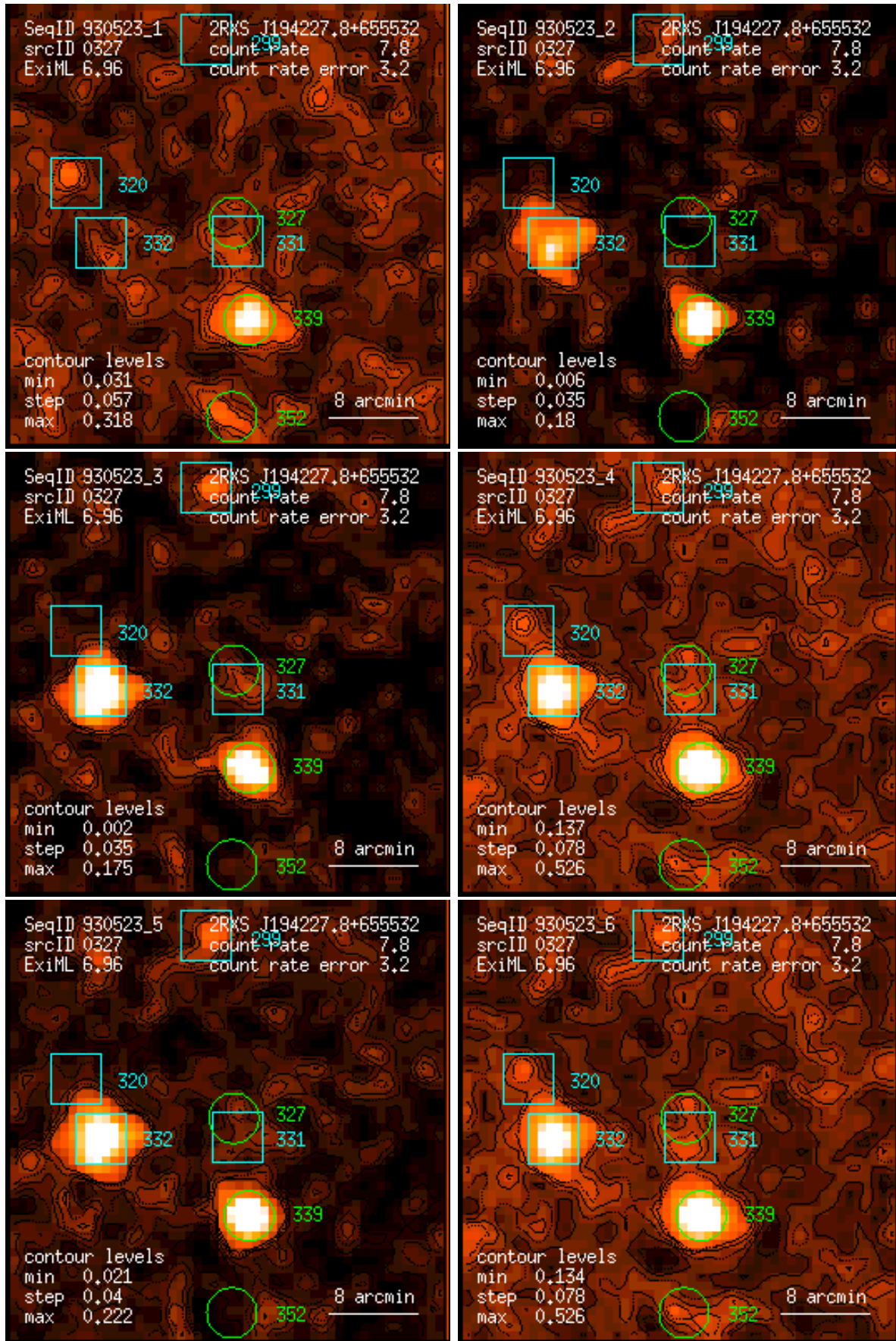
Figure 327: RASS 930523: detection 0327: band rate images, Gaussian filter: (1) PSPC channels 11 – 41, (2) 52 – 90, (3) 91 – 201, (4) 11 – 235, (5) 52 – 201, (6) 11 – 201. Broad band rates in counts/ks. Band rate contour levels in counts/ks/arcmin 2 .
