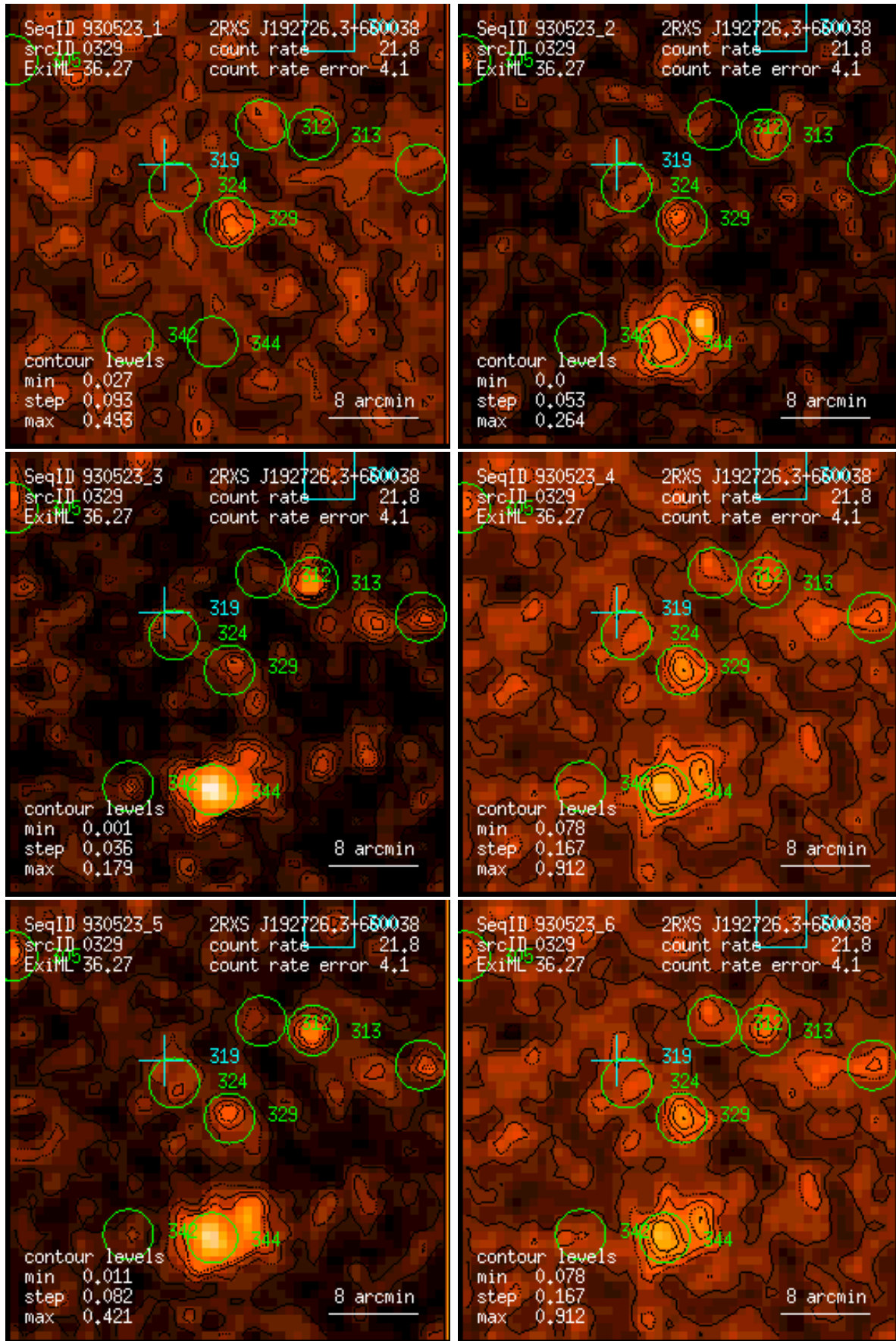
Figure 329: RASS 930523: detection 0329: band rate images, Gaussian filter: (1) PSPC channels 11 – 41, (2) 52 – 90, (3) 91 – 201, (4) 11 – 235, (5) 52 – 201, (6) 11 – 201. Broad band rates in counts/ks. Band rate contour levels in counts/ks/arcmin 2 .
