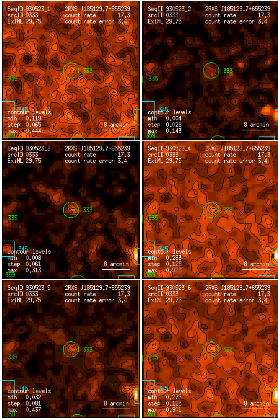
Figure 333: RASS 930523: detection 0333: band rate images, Gaussian filter: (1) PSPC channels 11 – 41, (2) 52 – 90, (3) 91 – 201, (4) 11 – 235, (5) 52 – 201, (6) 11 – 201. Broad band rates in counts/ks. Band rate contour levels in counts/ks/arcmin 2 .
