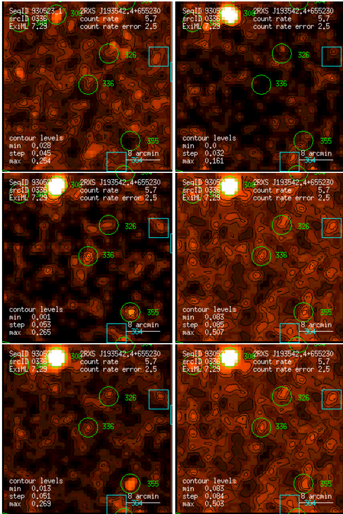
Figure 336: RASS 930523: detection 0336: band rate images, Gaussian filter: (1) PSPC channels 11 – 41, (2) 52 – 90, (3) 91 – 201, (4) 11 – 235, (5) 52 – 201, (6) 11 – 201. Broad band rates in counts/ks. Band rate contour levels in counts/ks/arcmin 2 .
