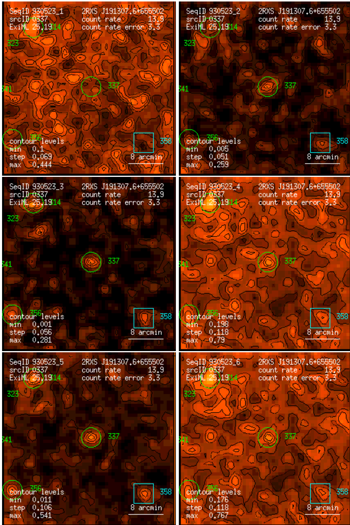
Figure 337: RASS 930523: detection 0337: band rate images, Gaussian filter: (1) PSPC channels 11 – 41, (2) 52 – 90, (3) 91 – 201, (4) 11 – 235, (5) 52 – 201, (6) 11 – 201. Broad band rates in counts/ks. Band rate contour levels in counts/ks/arcmin 2 .
