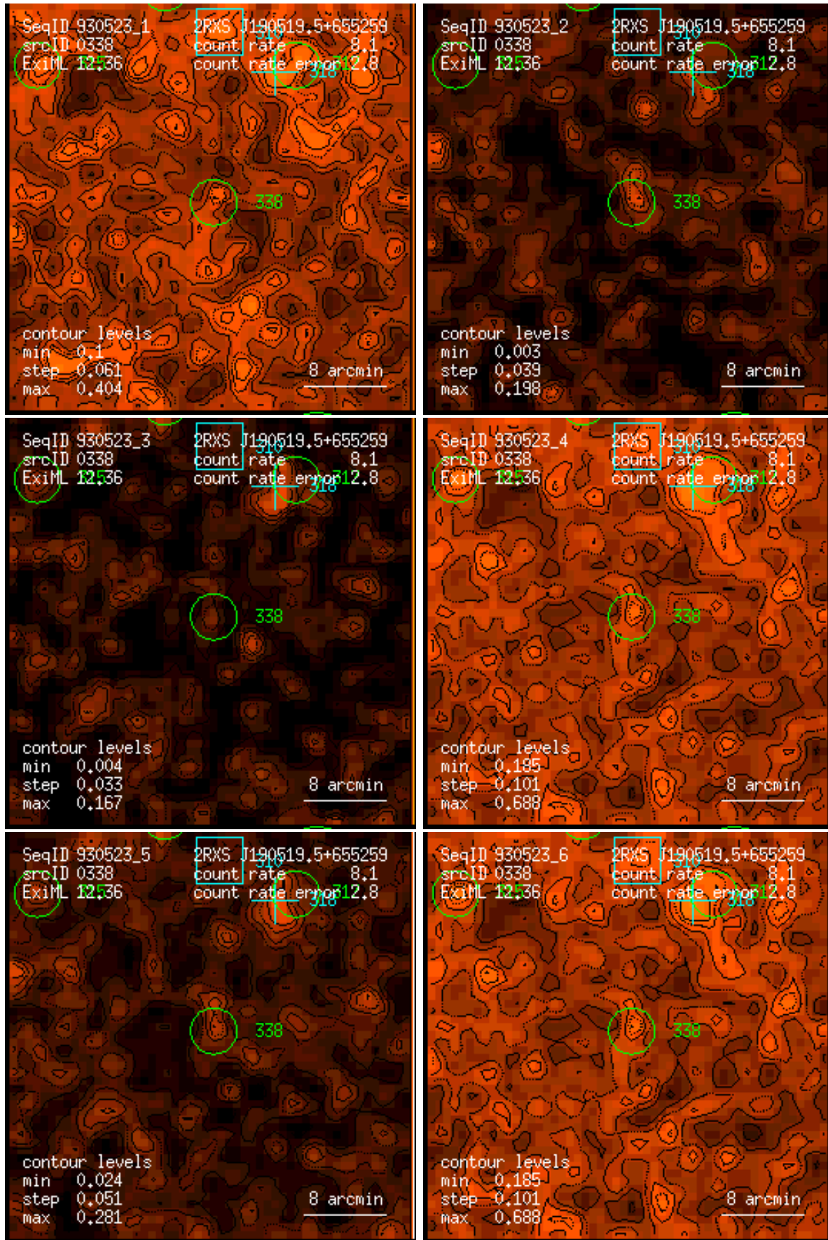
Figure 338: RASS 930523: detection 0338: band rate images, Gaussian filter: (1) PSPC channels 11 – 41, (2) 52 – 90, (3) 91 – 201, (4) 11 – 235, (5) 52 – 201, (6) 11 – 201. Broad band rates in counts/ks. Band rate contour levels in counts/ks/arcmin 2 .
