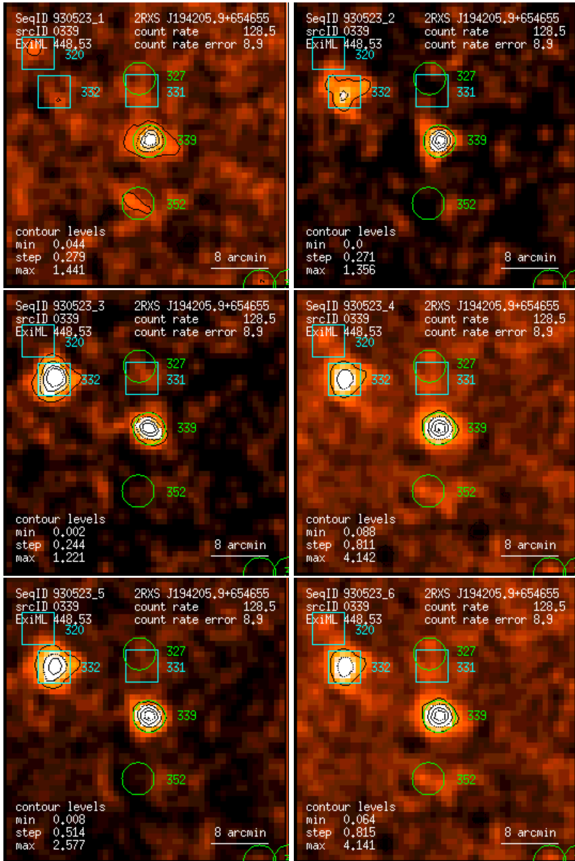
Figure 339: RASS 930523: detection 0339: band rate images, Gaussian filter: (1) PSPC channels 11 – 41, (2) 52 – 90, (3) 91 – 201, (4) 11 – 235, (5) 52 – 201, (6) 11 – 201. Broad band rates in counts/ks. Band rate contour levels in counts/ks/arcmin 2 .
