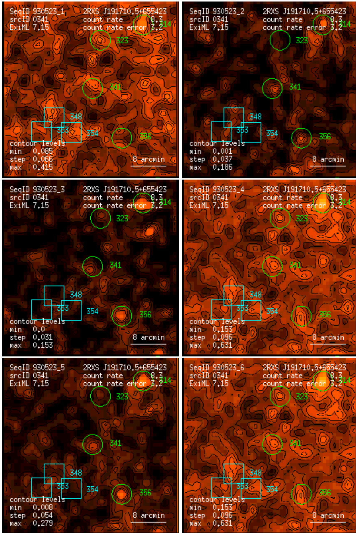
Figure 341: RASS 930523: detection 0341: band rate images, Gaussian filter: (1) PSPC channels 11 – 41, (2) 52 – 90, (3) 91 – 201, (4) 11 – 235, (5) 52 – 201, (6) 11 – 201. Broad band rates in counts/ks. Band rate contour levels in counts/ks/arcmin 2 .
