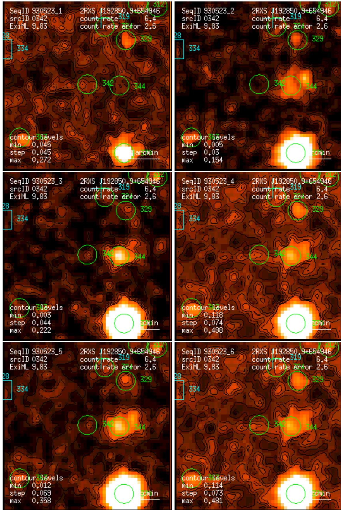
Figure 342: RASS 930523: detection 0342: band rate images, Gaussian filter: (1) PSPC channels 11 – 41, (2) 52 – 90, (3) 91 – 201, (4) 11 – 235, (5) 52 – 201, (6) 11 – 201. Broad band rates in counts/ks. Band rate contour levels in counts/ks/arcmin 2 .
