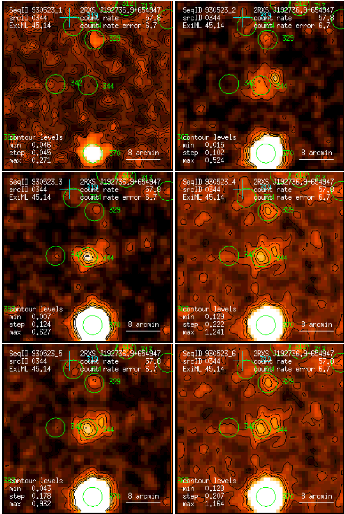
Figure 344: RASS 930523: detection 0344: band rate images, Gaussian filter: (1) PSPC channels 11 – 41, (2) 52 – 90, (3) 91 – 201, (4) 11 – 235, (5) 52 – 201, (6) 11 – 201. Broad band rates in counts/ks. Band rate contour levels in counts/ks/arcmin 2 .
