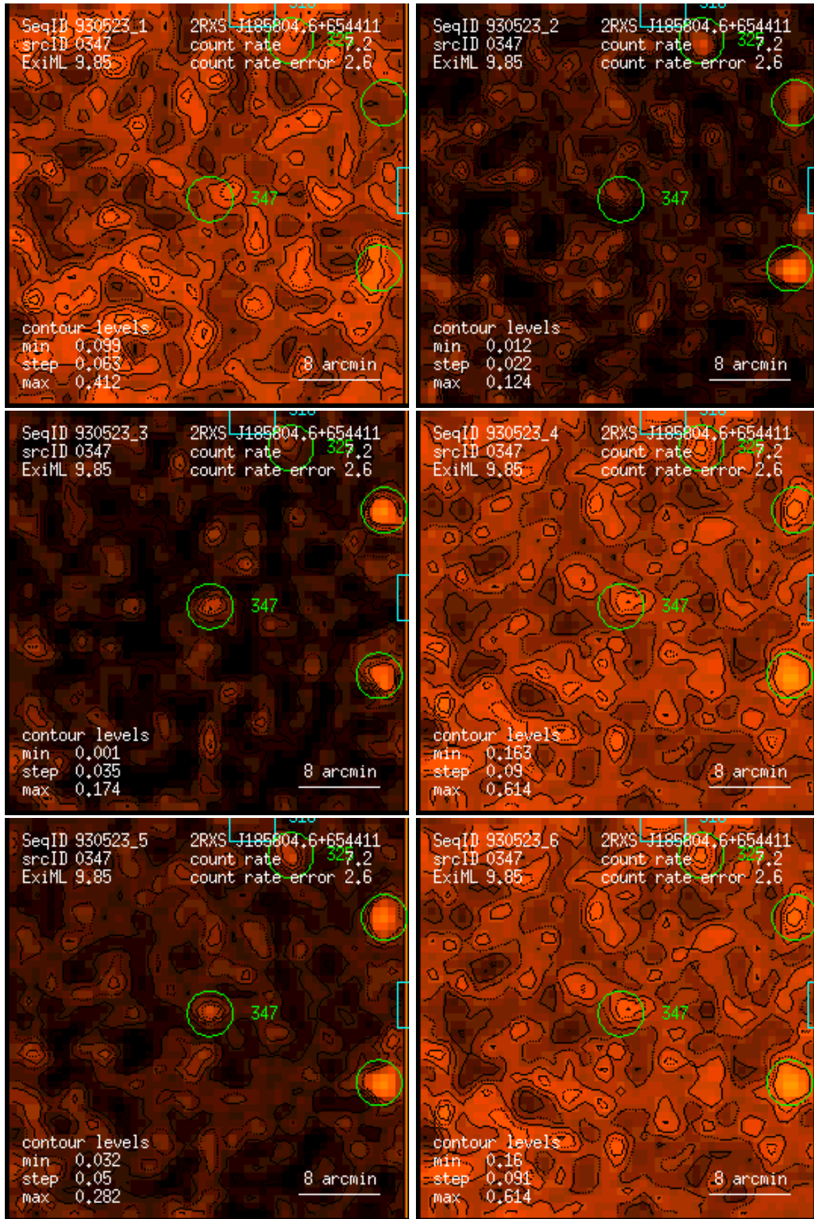
Figure 347: RASS 930523: detection 0347: band rate images, Gaussian filter: (1) PSPC channels 11 – 41, (2) 52 – 90, (3) 91 – 201, (4) 11 – 235, (5) 52 – 201, (6) 11 – 201. Broad band rates in counts/ks. Band rate contour levels in counts/ks/arcmin 2 .
