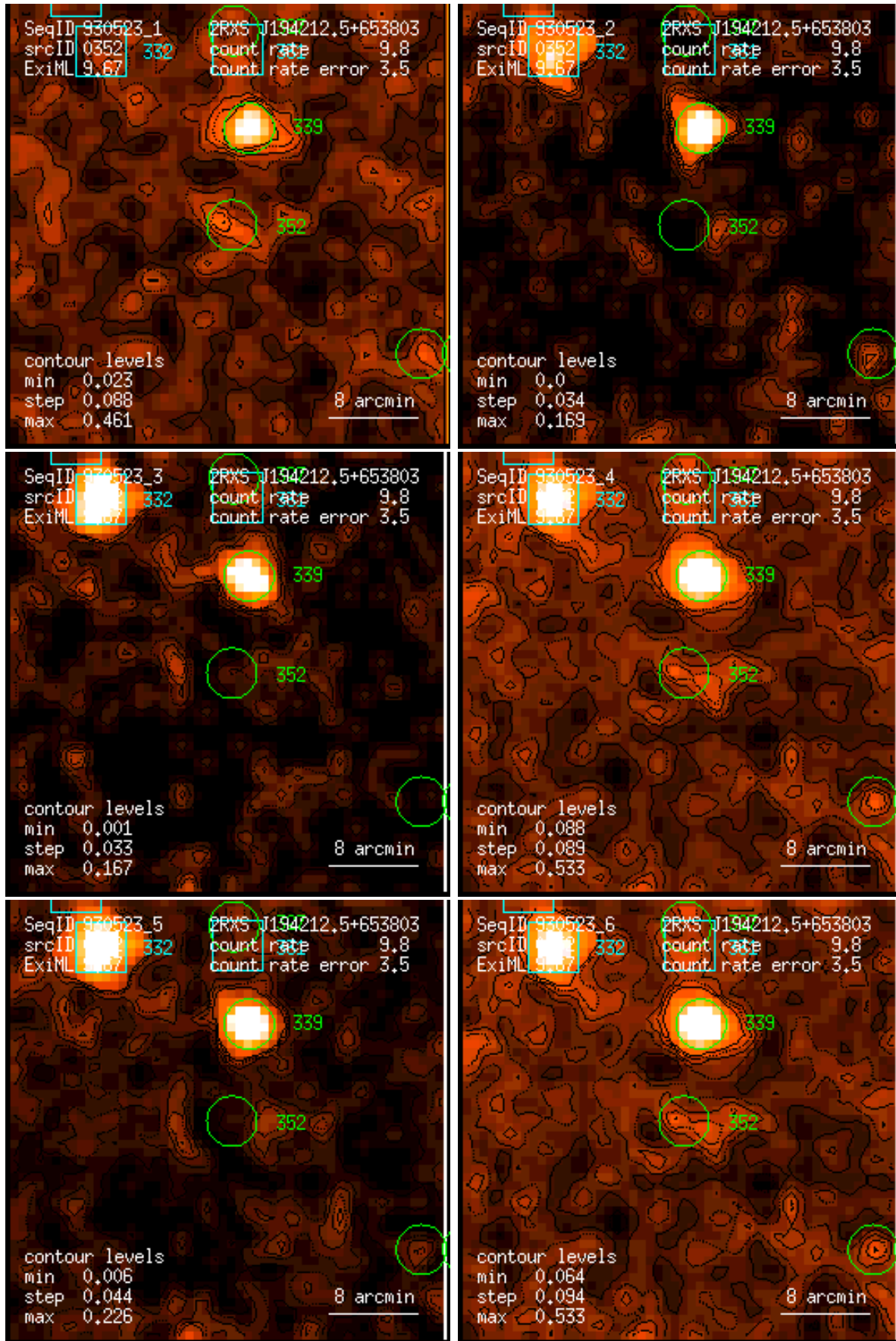
Figure 352: RASS 930523: detection 0352: band rate images, Gaussian filter: (1) PSPC channels 11 – 41, (2) 52 – 90, (3) 91 – 201, (4) 11 – 235, (5) 52 – 201, (6) 11 – 201. Broad band rates in counts/ks. Band rate contour levels in counts/ks/arcmin 2 .
