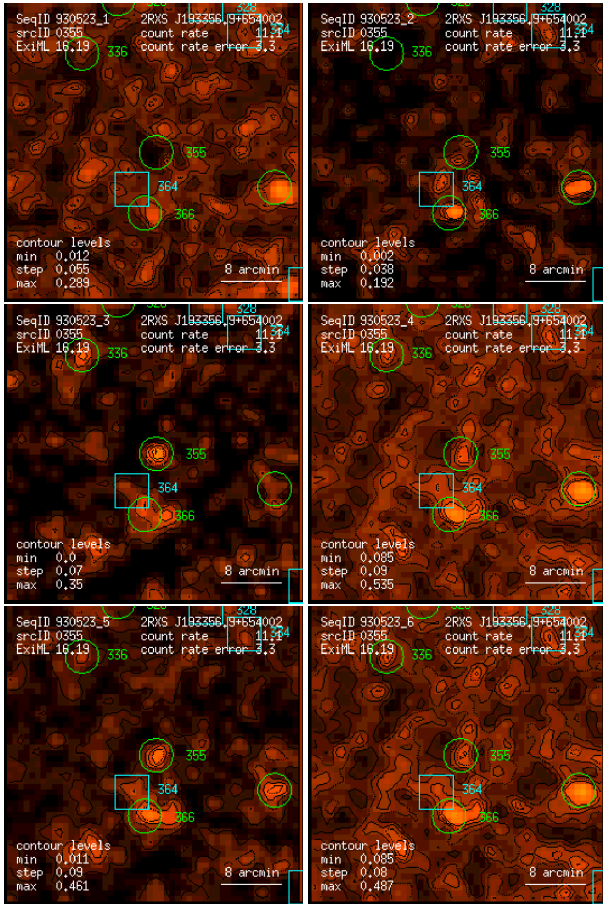
Figure 355: RASS 930523: detection 0355: band rate images, Gaussian filter: (1) PSPC channels 11 – 41, (2) 52 – 90, (3) 91 – 201, (4) 11 – 235, (5) 52 – 201, (6) 11 – 201. Broad band rates in counts/ks. Band rate contour levels in counts/ks/arcmin 2 .
