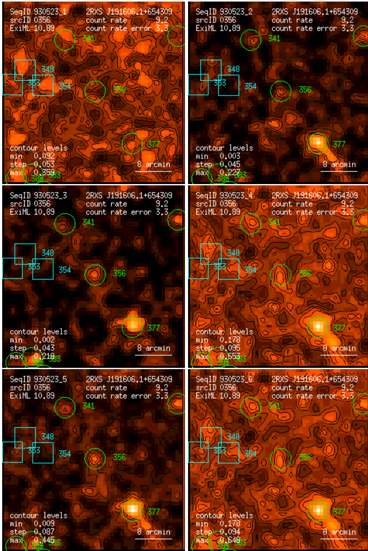
Figure 356: RASS 930523: detection 0356: band rate images, Gaussian filter: (1) PSPC channels 11 – 41, (2) 52 – 90, (3) 91 – 201, (4) 11 – 235, (5) 52 – 201, (6) 11 – 201. Broad band rates in counts/ks. Band rate contour levels in counts/ks/arcmin 2 .
