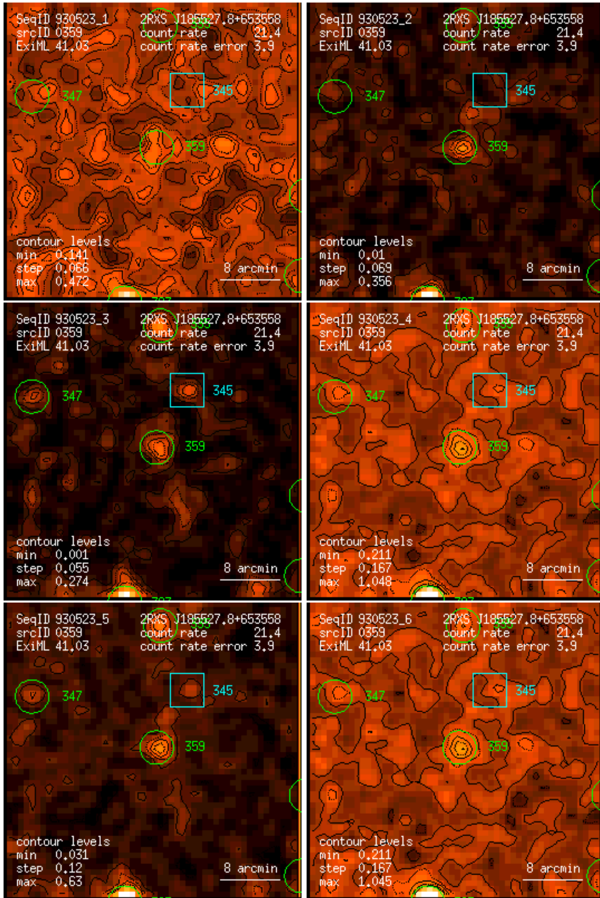
Figure 359: RASS 930523: detection 0359: band rate images, Gaussian filter: (1) PSPC channels 11 – 41, (2) 52 – 90, (3) 91 – 201, (4) 11 – 235, (5) 52 – 201, (6) 11 – 201. Broad band rates in counts/ks. Band rate contour levels in counts/ks/arcmin 2 .
