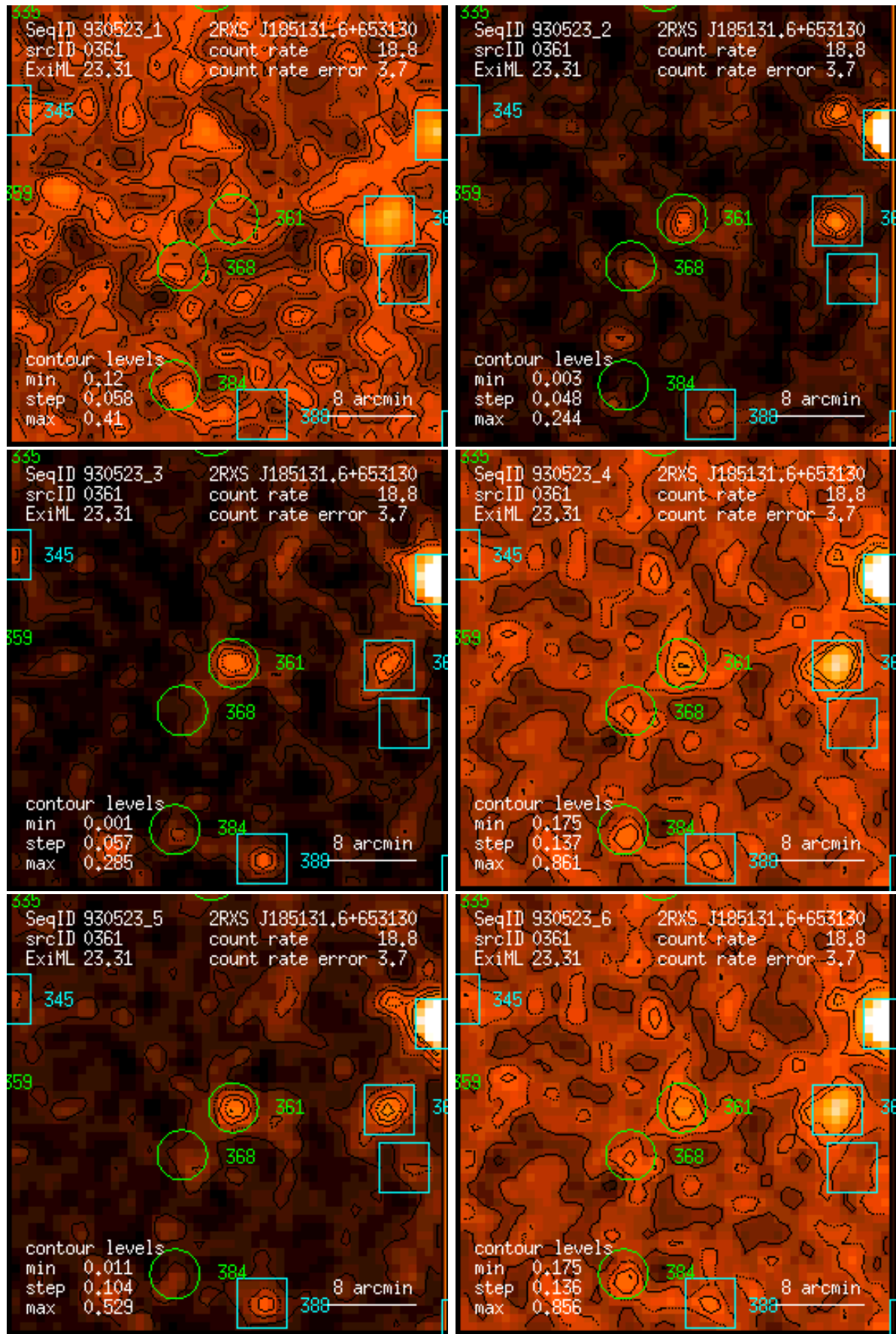
Figure 361: RASS 930523: detection 0361: band rate images, Gaussian filter: (1) PSPC channels 11 – 41, (2) 52 – 90, (3) 91 – 201, (4) 11 – 235, (5) 52 – 201, (6) 11 – 201. Broad band rates in counts/ks. Band rate contour levels in counts/ks/arcmin 2 .
