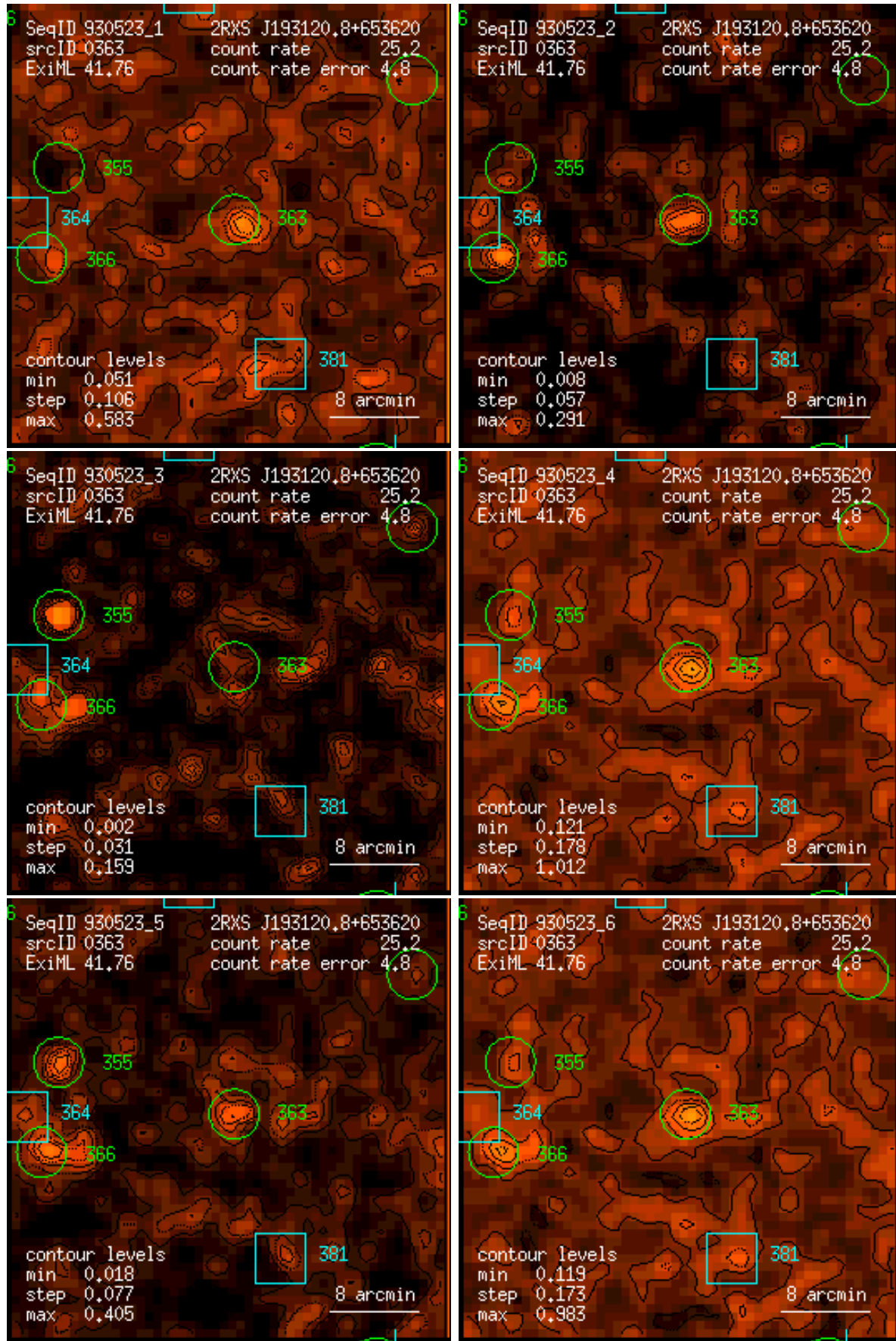
Figure 363: RASS 930523: detection 0363: band rate images, Gaussian filter: (1) PSPC channels 11 – 41, (2) 52 – 90, (3) 91 – 201, (4) 11 – 235, (5) 52 – 201, (6) 11 – 201. Broad band rates in counts/ks. Band rate contour levels in counts/ks/arcmin 2 .
