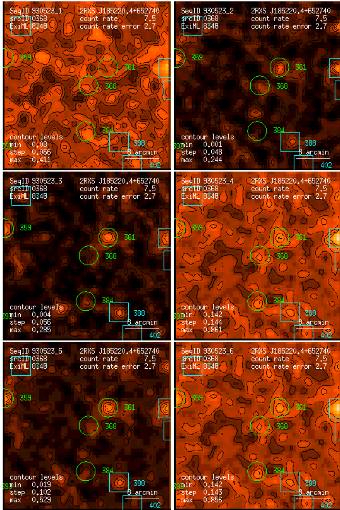
Figure 368: RASS 930523: detection 0368: band rate images, Gaussian filter: (1) PSPC channels 11 – 41, (2) 52 – 90, (3) 91 – 201, (4) 11 – 235, (5) 52 – 201, (6) 11 – 201. Broad band rates in counts/ks. Band rate contour levels in counts/ks/arcmin 2 .
